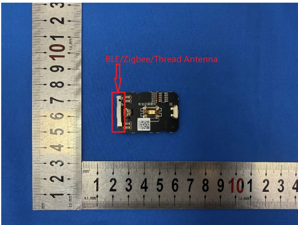
Photo 6: Internal View for BLE/Zigbee/Thread Antenna
