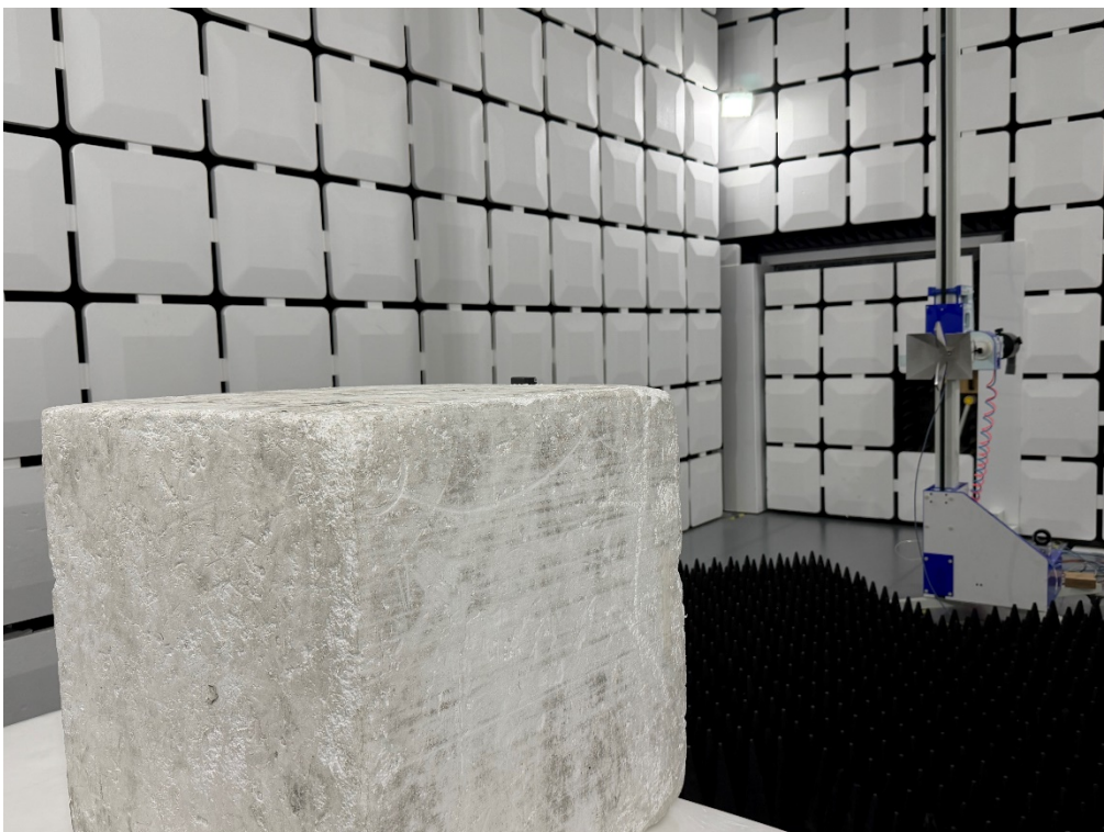
Description: Radiated Emission Test Setup for Above 1-18GHz
