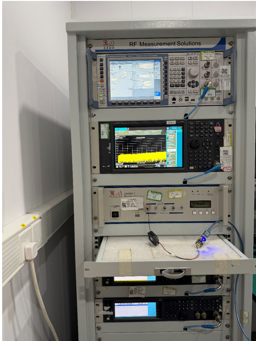
Description: Conducted Test Setup Photo
