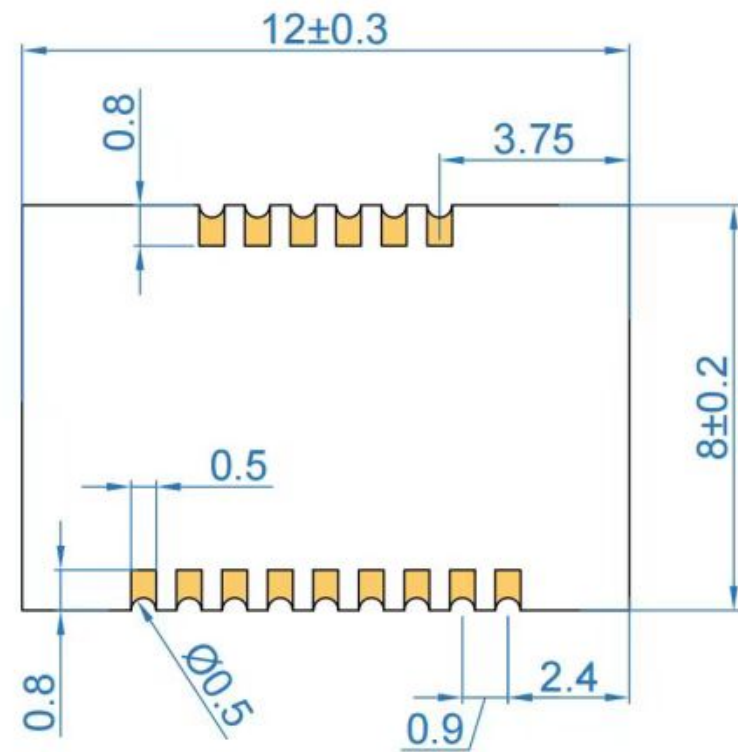
Bottom View
