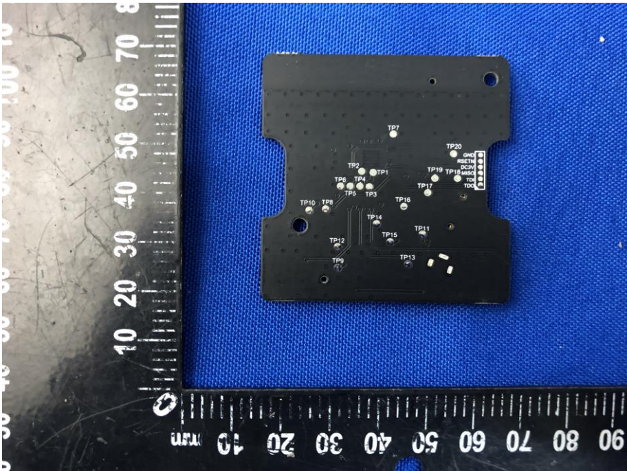
MAIN BOARD BACK VIEW (WXKG03LM)
