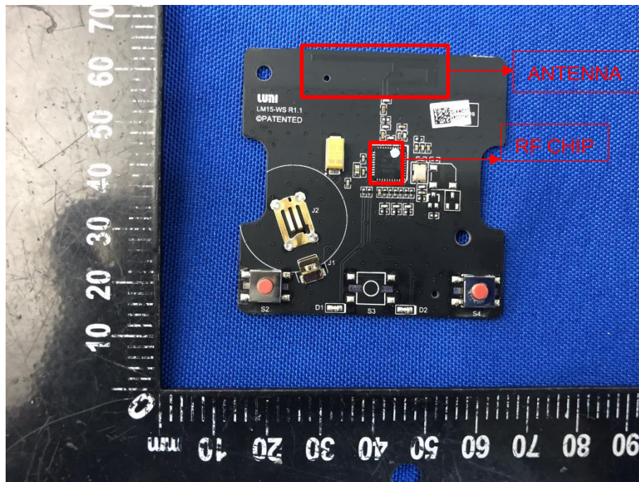
MAIN BOARD FRONT VIEW (WXKG02LM)
