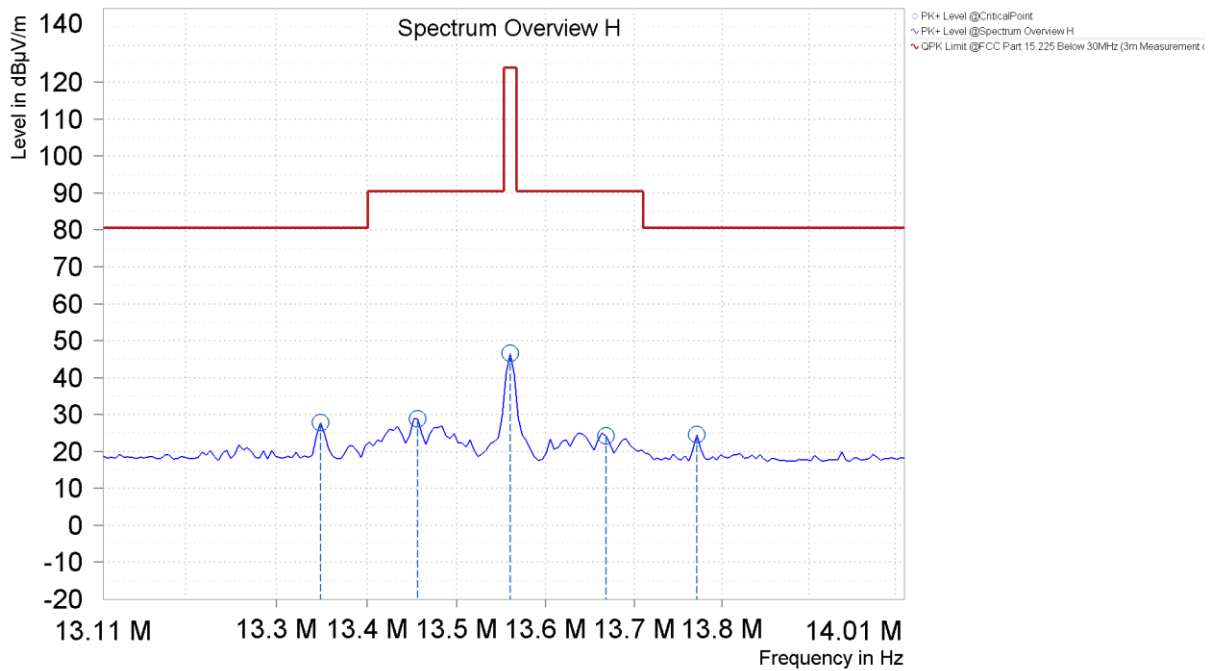
Figure 9. In-Band Emission Mask (Coplanar Loop)
