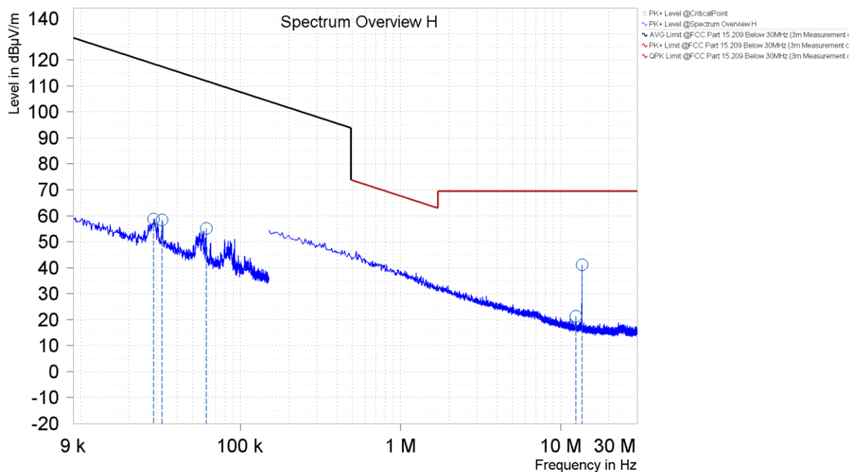
Figure 11. Out of Band Emissions Below 30MHz (Coplanar Loop)
