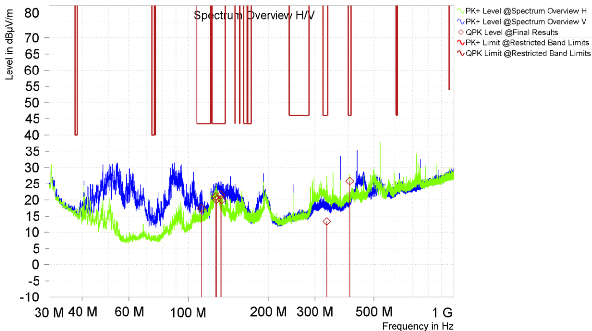
Figure 13. Out of Band Emissions Above 30MHz (Vertical and Horizontal Polarity)
