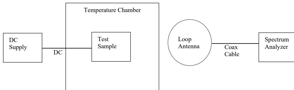
Figure 14. Temperature Stability Test Setup
