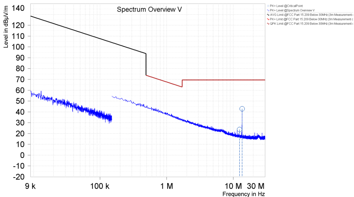
Figure 12. Out of Band Emissions Below 30MHz (Coaxial Loop)
