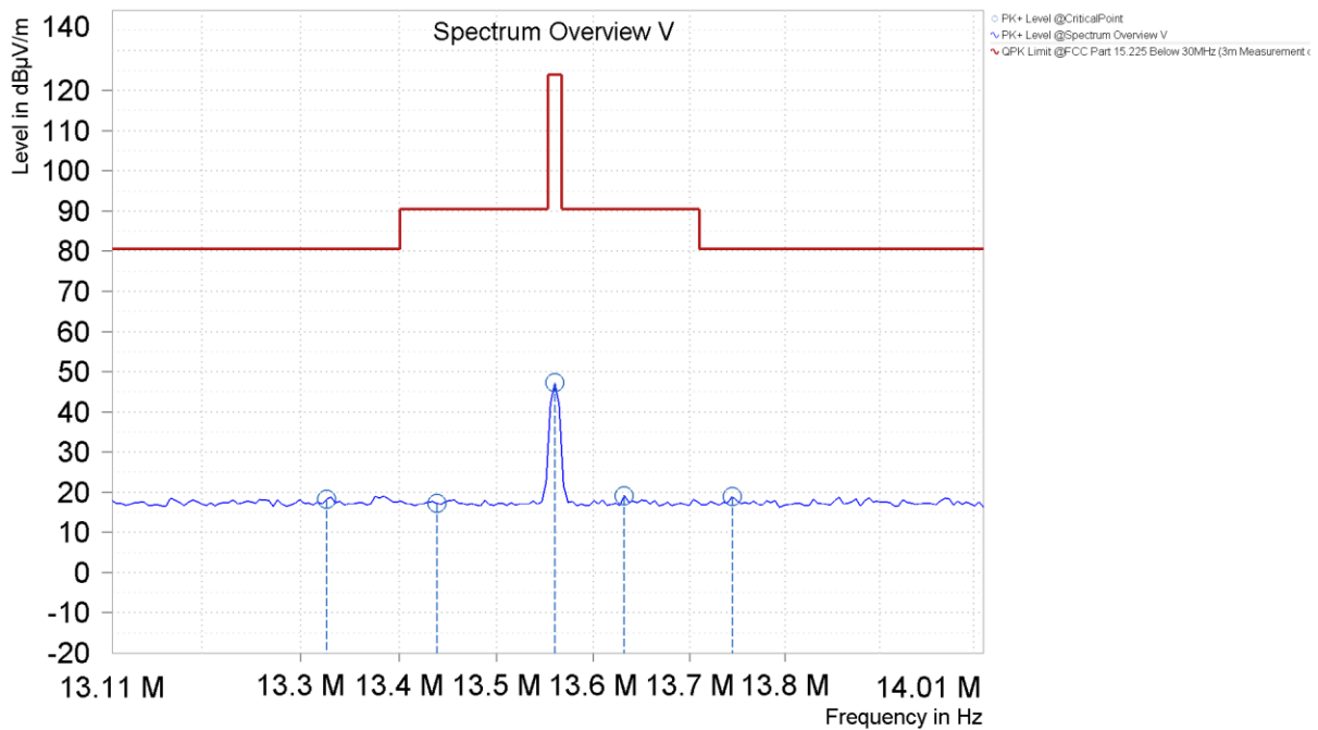
Figure 10. In-Band Emission Mask (Coaxial Loop)
