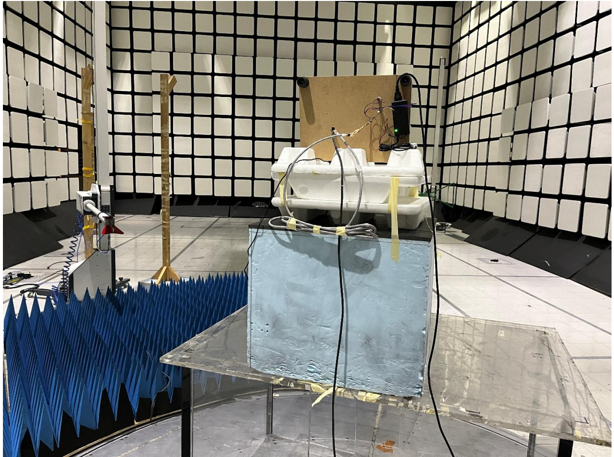
Radiated Emissions Above 1GHz (Back View)
