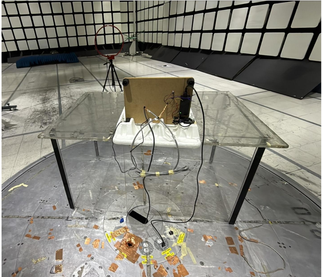
Radiated Emissions Below 30MHz (Back View)
