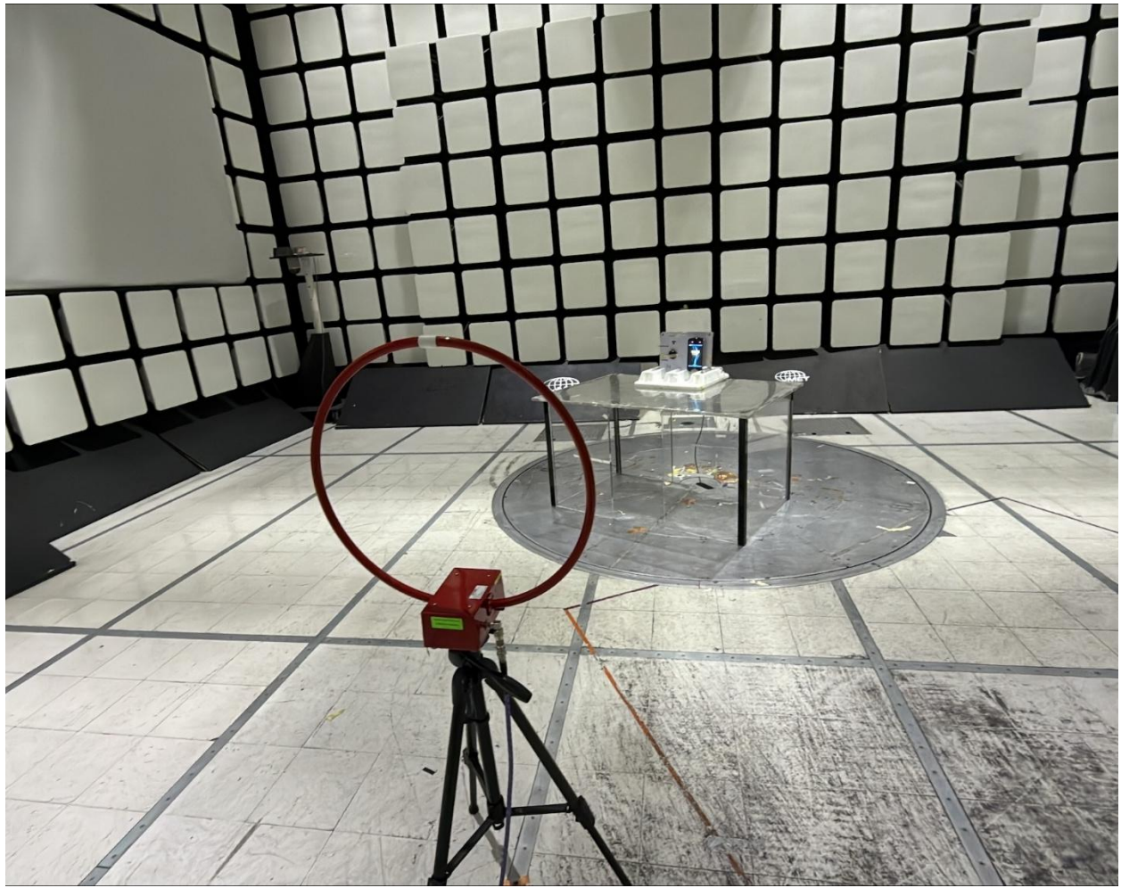
Radiated Emissions Below 30MHz (Front View)
