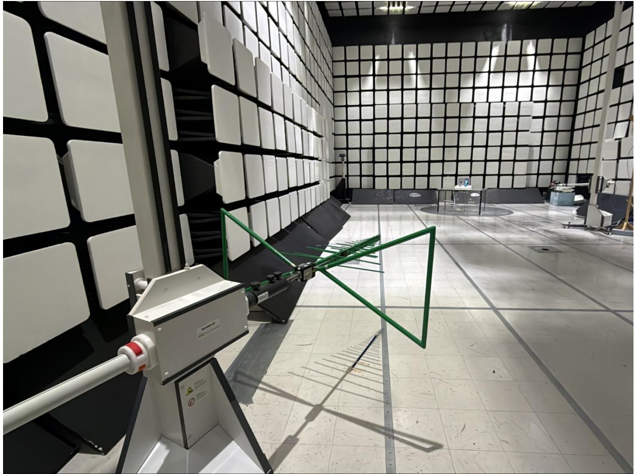
Radiated Emissions 30MHz - 1GHz (Antenna View)
