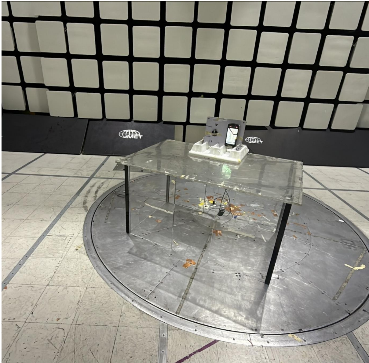
Radiated Emissions 30MHz - 1GHz (Front View)
