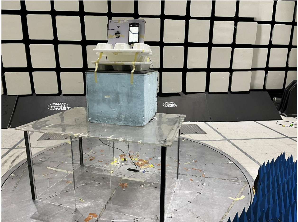
Radiated Emissions Above 1GHz (Front View)
