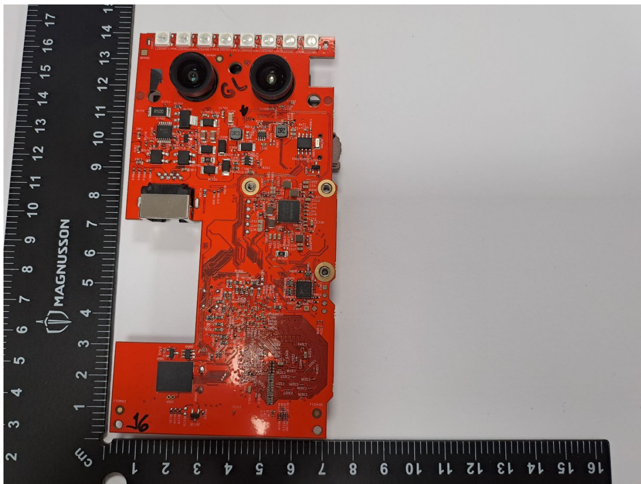
Main PCB Rear View out of housing
