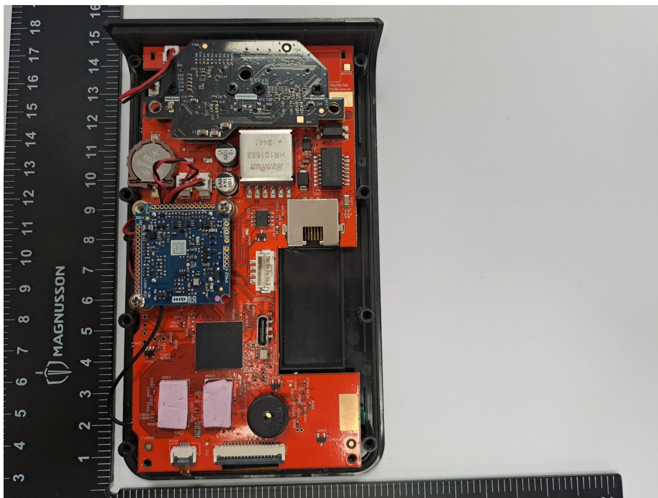
Main PCB Front View in housing
