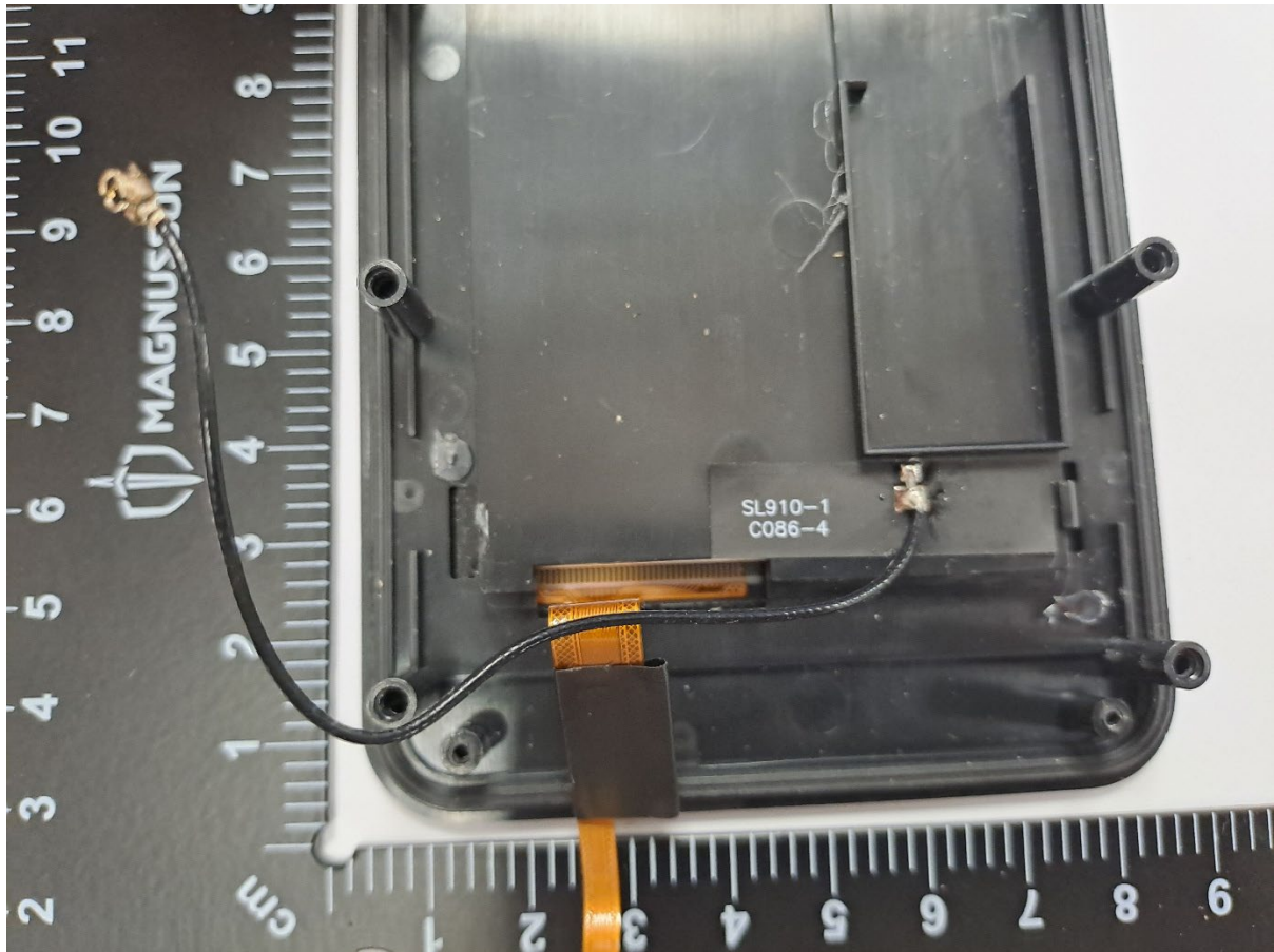
Bluetooth Antenna location in housing
