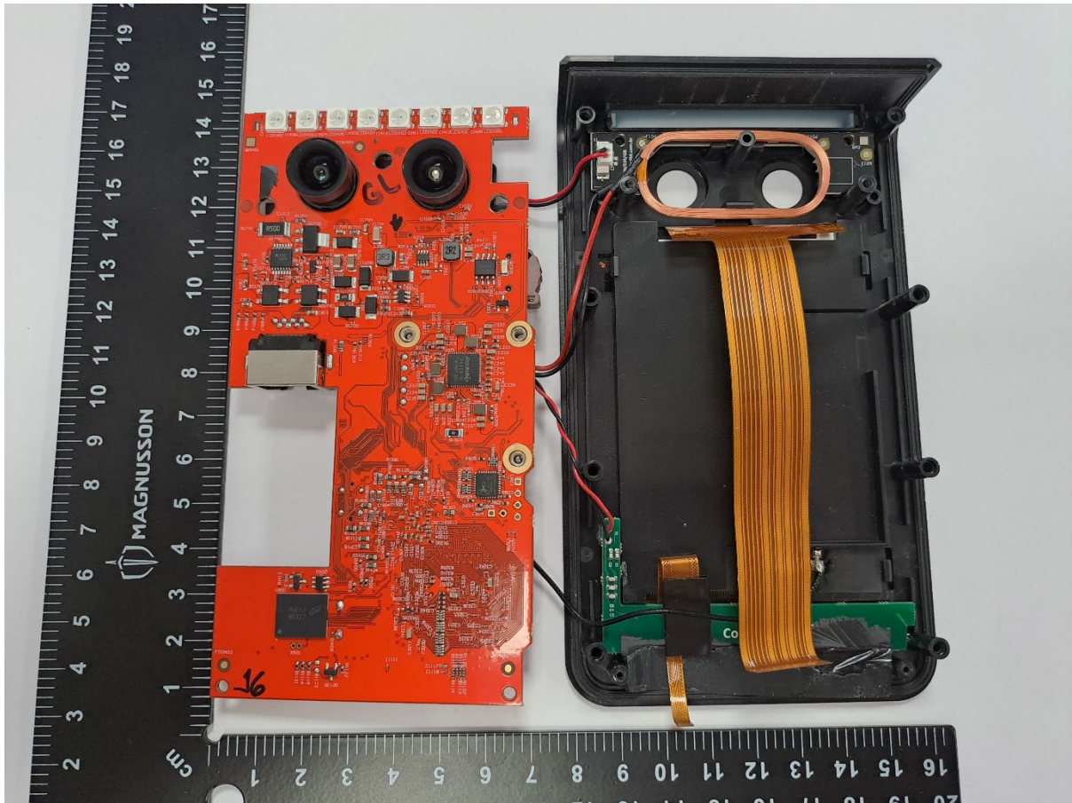
Main PCB removed from housing showing LCD ribbon, and all antenna's
