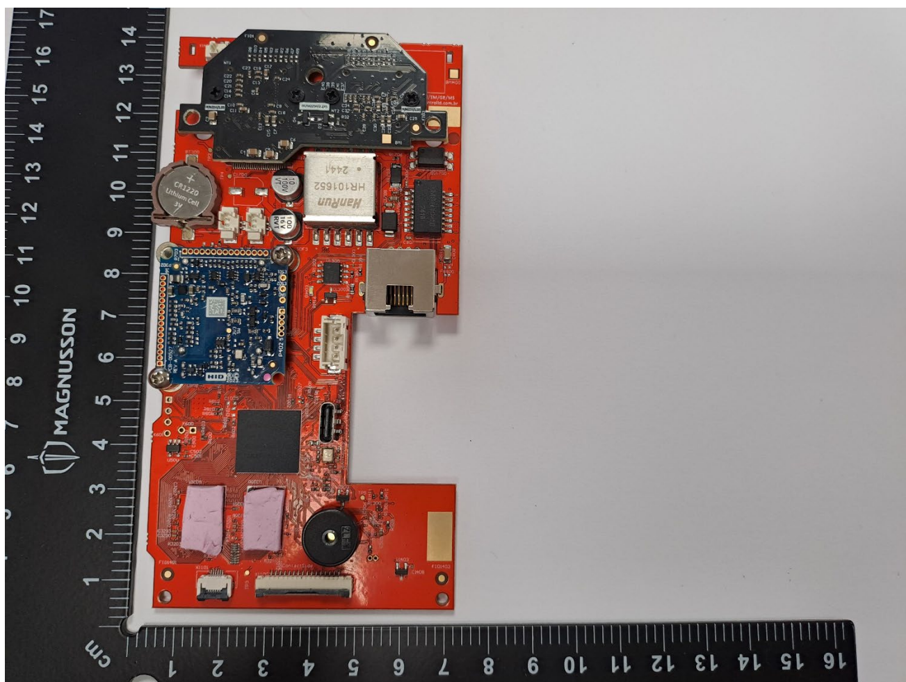
Main PCB front view out of the housing
