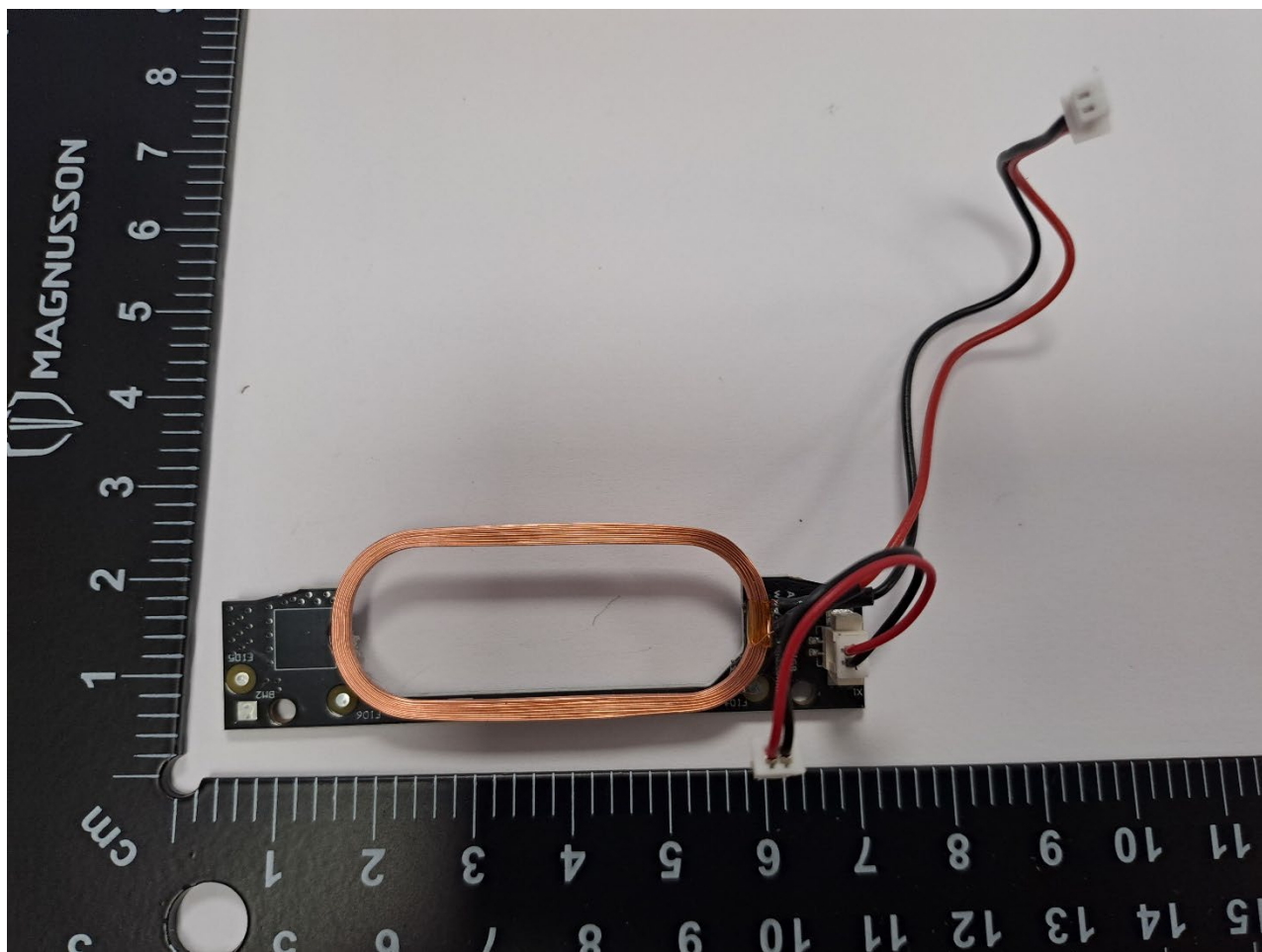
LF (125kHz) antenna coil on LED PCB
