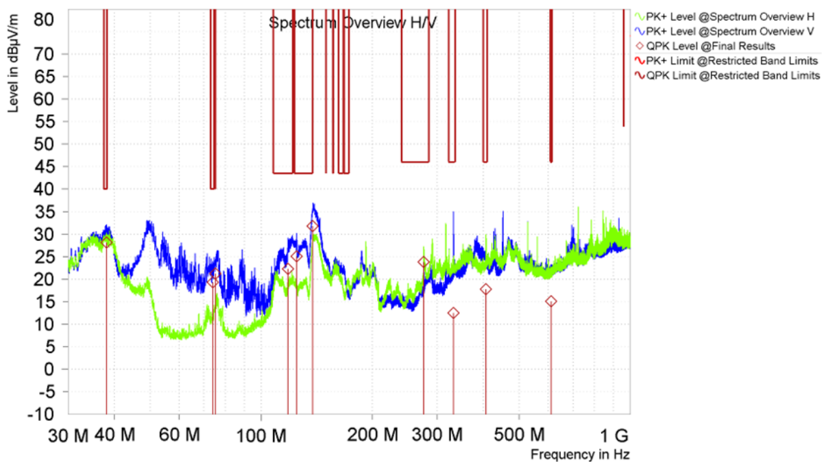
Figure 13. Out of Band Emissions Above 30MHz (Vertical and Horizontal Polarity)
