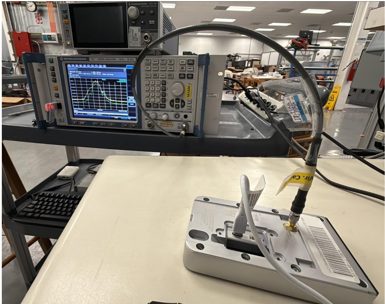
Conducted Antenna Port Measurements
