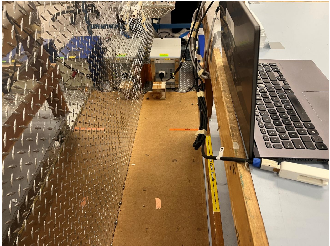
Conducted Emissions (Side View)
