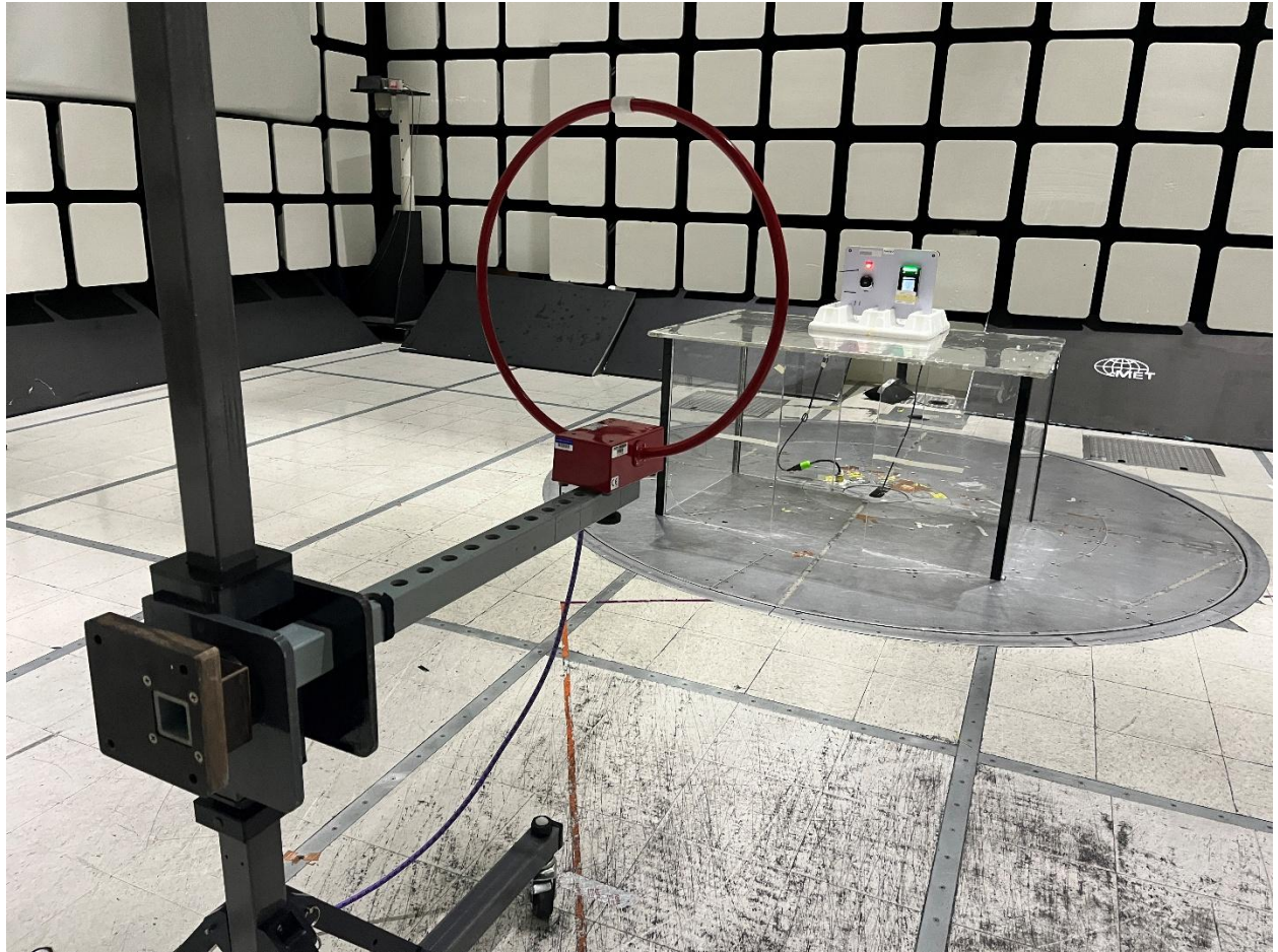
Radiated Emissions Below 30MHz (Antenna Side)
