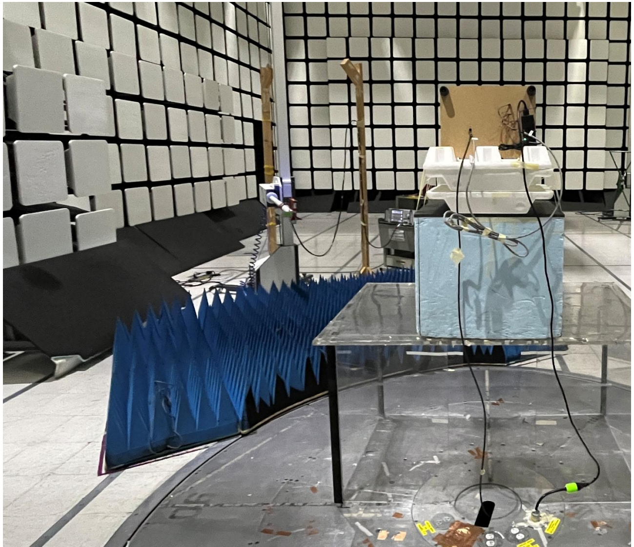
Radiated Emissions Above 1GHz (Back Side)
