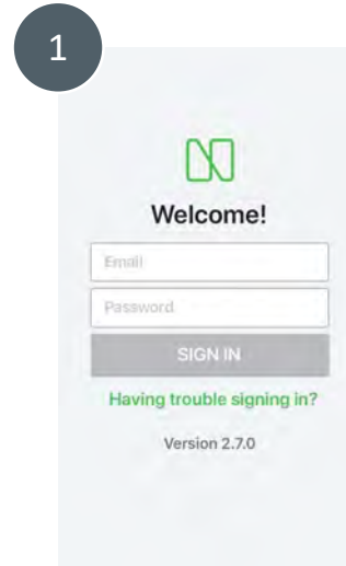
Login screen
