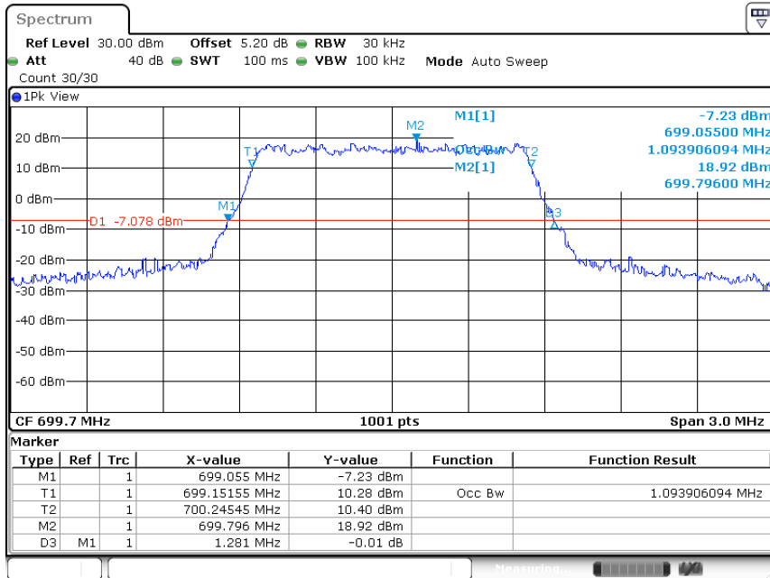
Band12-1.4MHz-QPSK-23017-6RB#0-1.094
