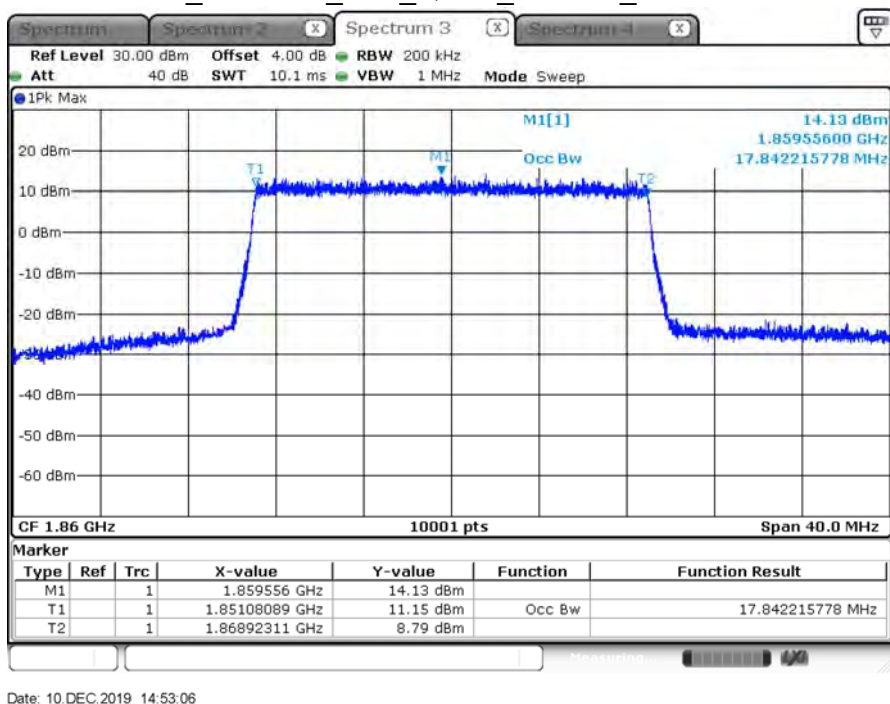
B2_CH18700_20M_QPSK_100RB0_99% BW
