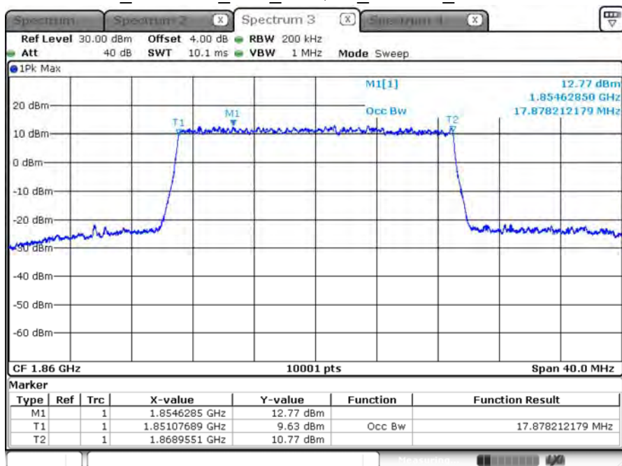
B2_CH18700_20M_16-QAM_100RB0_99% BW
