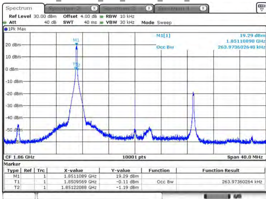
B2_CH18700_20M_16-QAM_1RB0_99% BW
