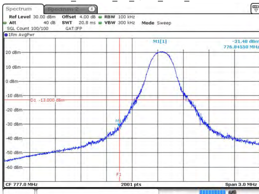
B13_CH23205_5M_QPSK_1RB0_150k
