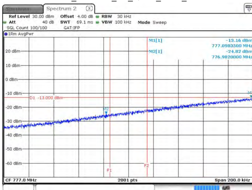
B13_CH23205_5M_QPSK_1RB0_15k
