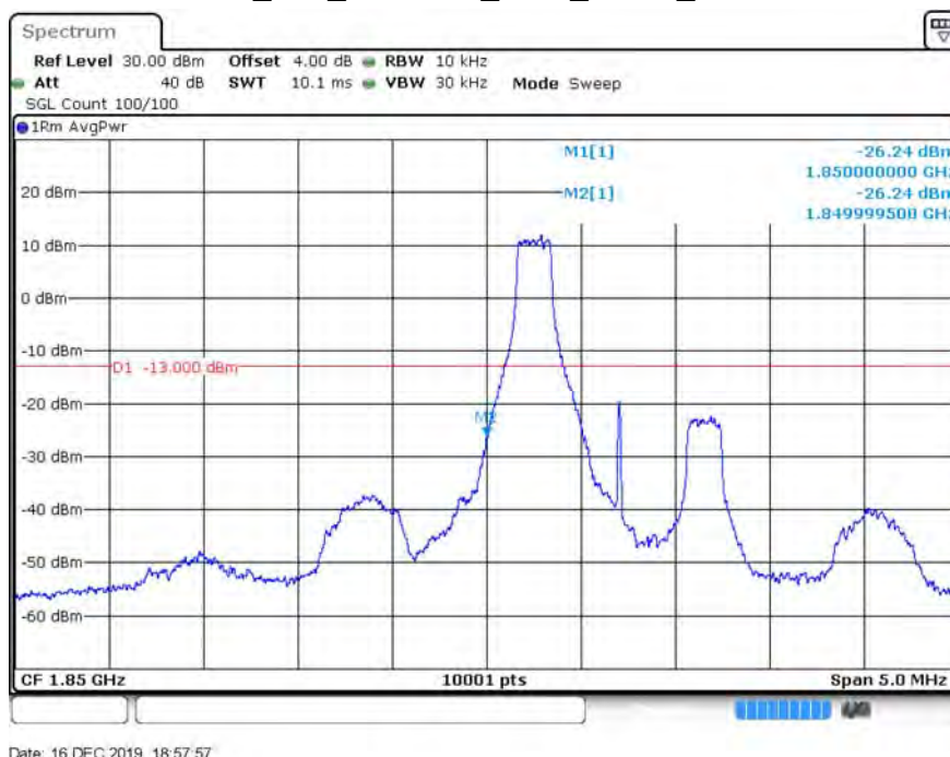
LTE_B25_CH26047_1.4M_QPSK_6RB0
