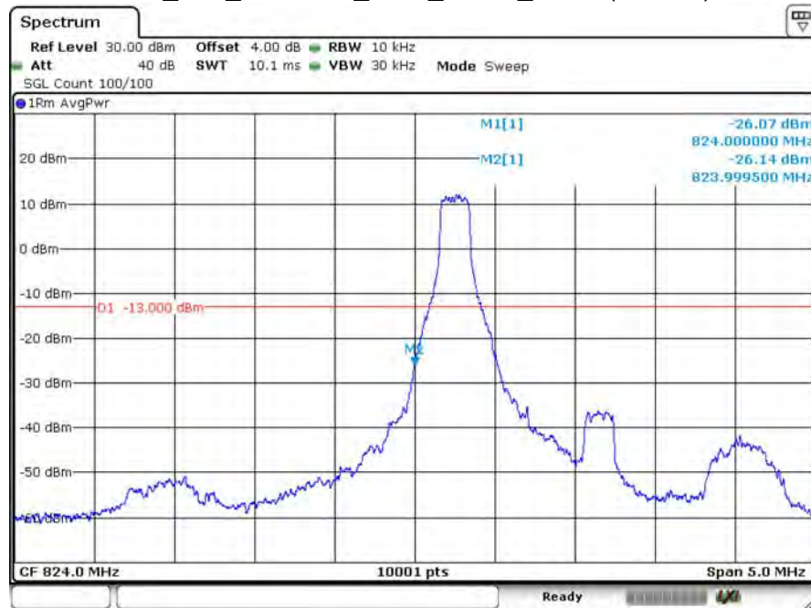
LTE_B26_CH26797_1.4M_QPSK_1RB0 (Part 22)
