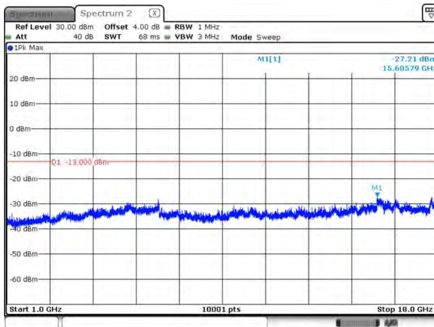
B5_CH20643_1.4M_1RB2_16-QAM_Above 1G
