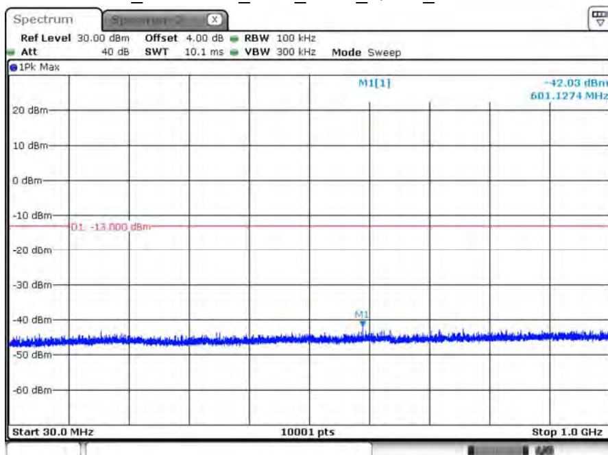
B66_CH131979_1.4M_1RB2_QPSK_Below 1G
