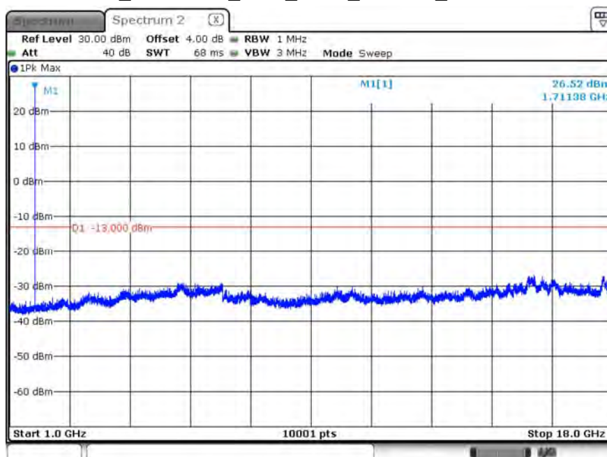
B66_CH131979_1.4M_1RB2_16-QAM_Above 1G
