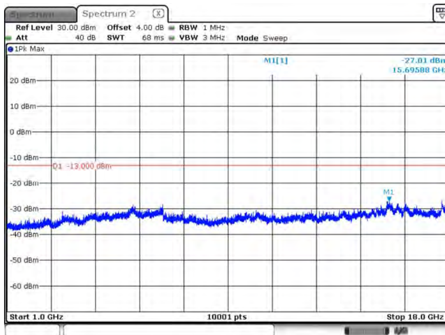
B13_CH23230_10M_1RB24_16-QAM_Above 1G
