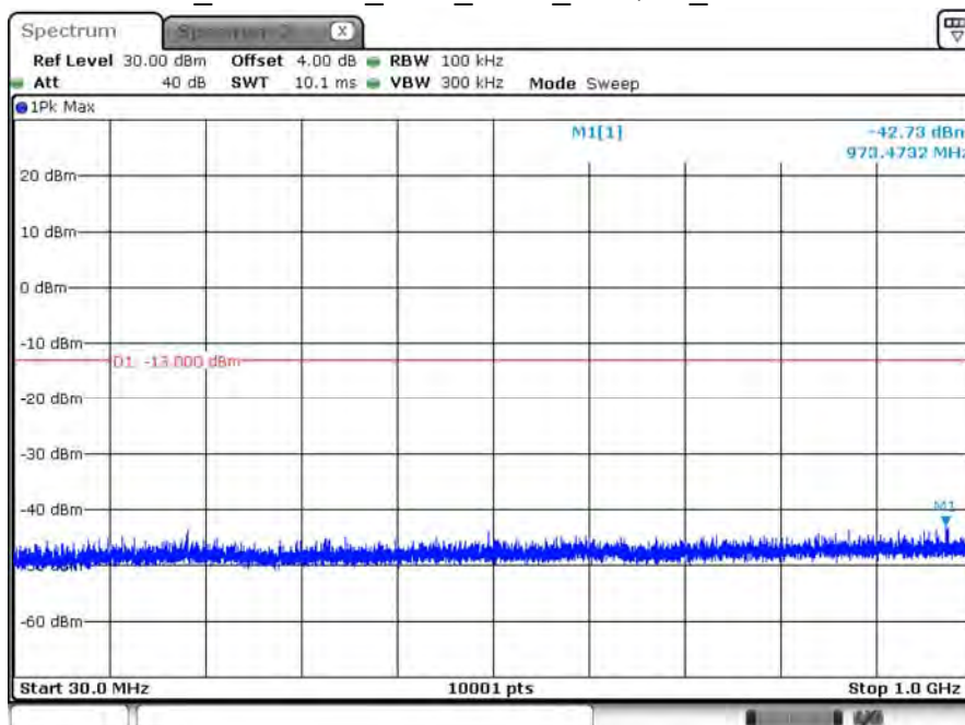
B66_CH131979_1.4M_1RB2_16-QAM_Below 1G
