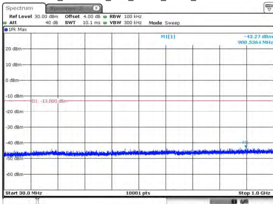
B66_CH132597_15M_1RB37_QPSK_Below 1G
