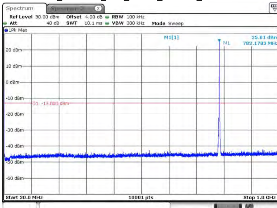
B13_CH23230_10M_1RB24_16-QAM_Below 1G
