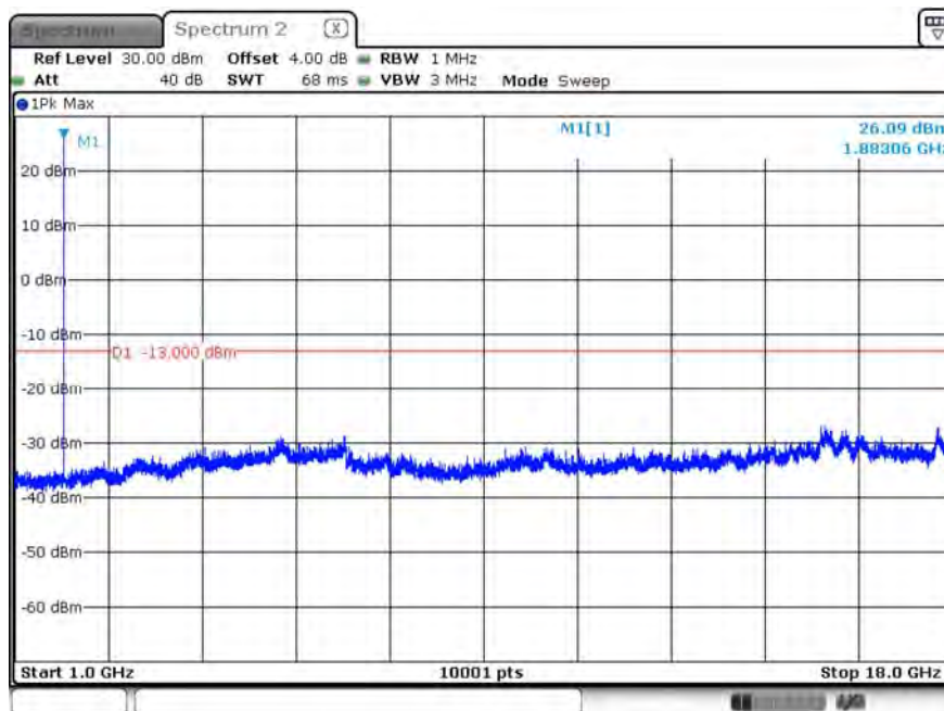
B25_CH26365_1.4M_1RB2_16-QAM_Above 1G
