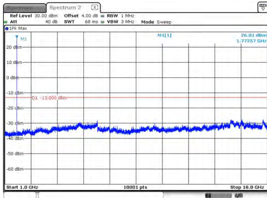
B66_CH132597_15M_1RB37_QPSK_Above 1G
