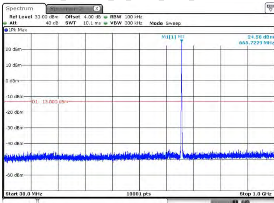
B71_CH113147_5M_1RB12_QPSK_Below 1G
