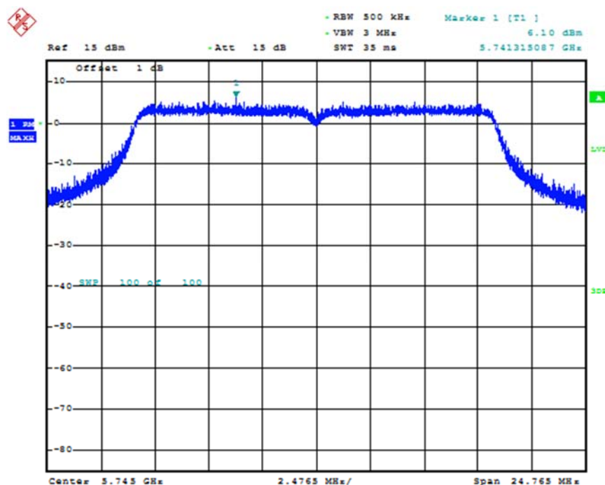
Fig. 1 Power Spectral Density (802.11a, Ch 149)
