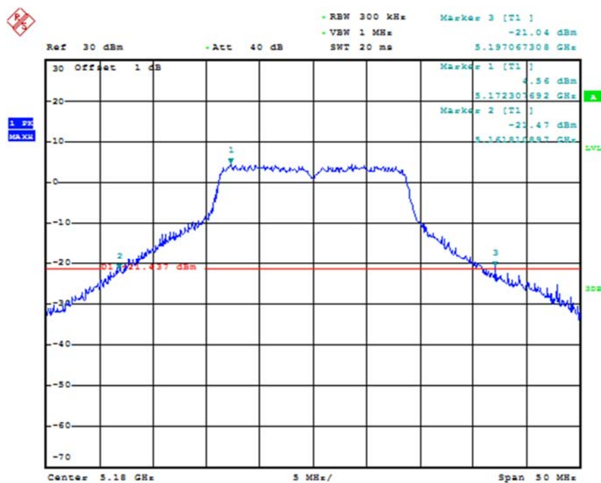
Fig. 12 Occupied 26dB Bandwidth (802.11n-HT20, 5180MHz)
