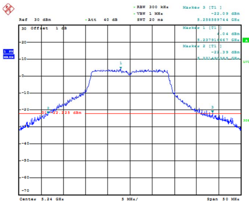
Fig. 14 Occupied 26dB Bandwidth (802.11n-HT20, 5240MHz)
