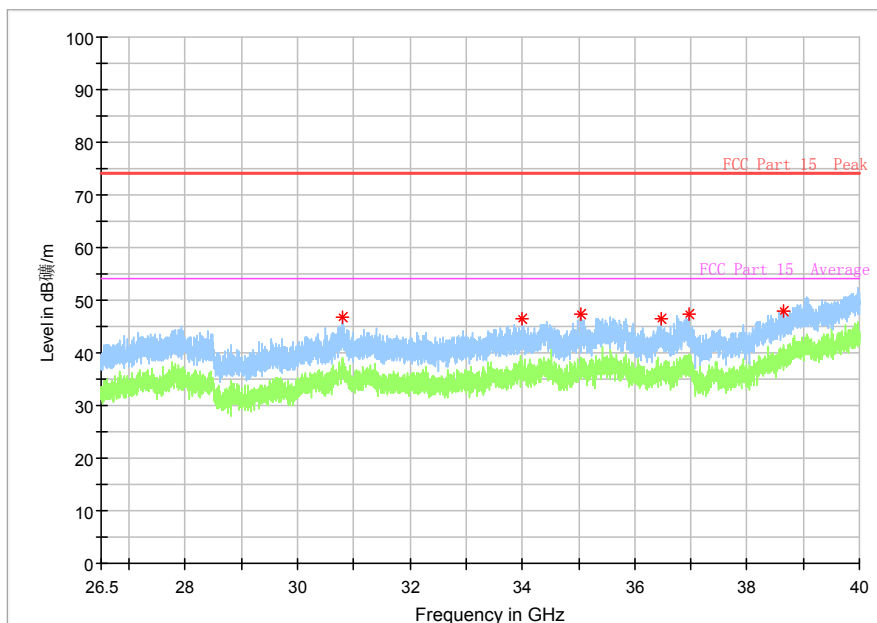
Fig. 46 Radiated Spurious Emission (802.11n-HT20, ch48, 26.5 GHz-40 GHz)
