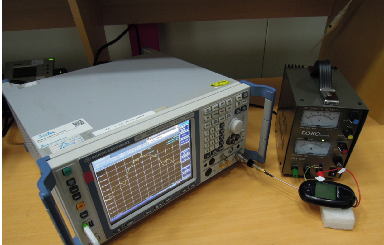
Photograph 6: Set-up for Conducted testing I
