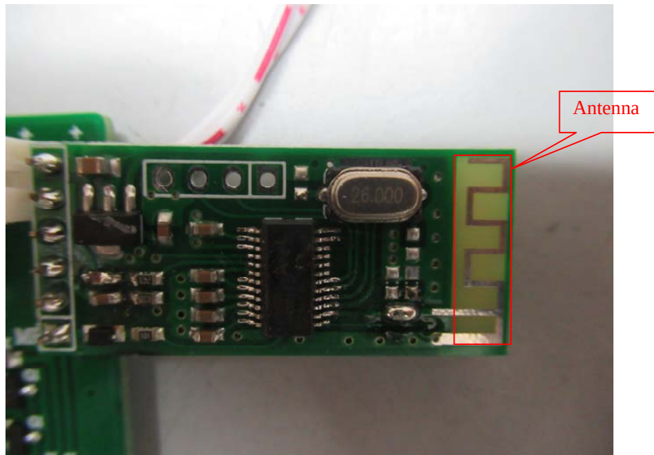
EUT – PCB-3 Chip View-2-Main Unit
