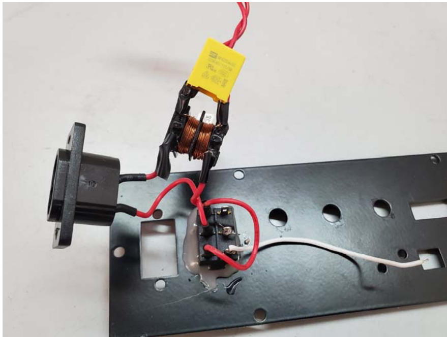
EUT – Cover off View-4-Main Unit
