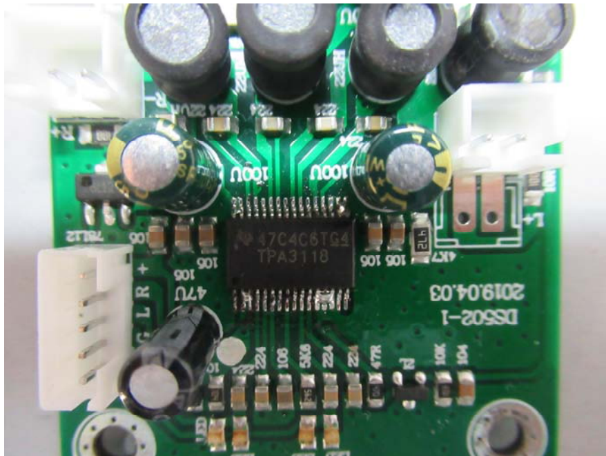
EUT – PCB-1 Chip View-2-Main Unit
