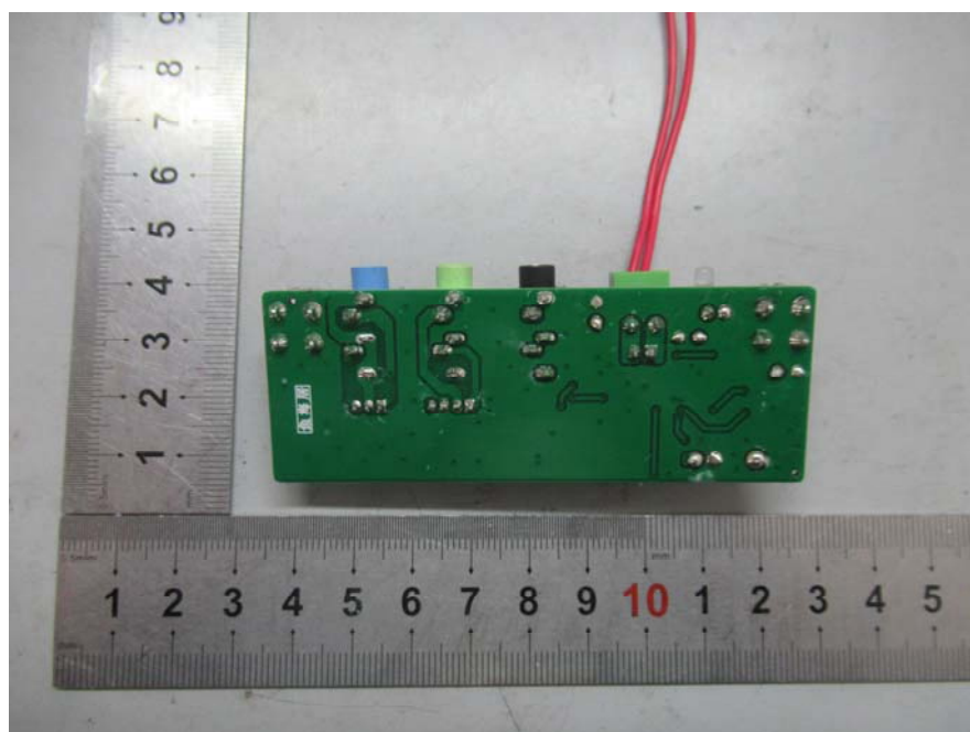
EUT – PCB-2 Bottom View-Main Unit
