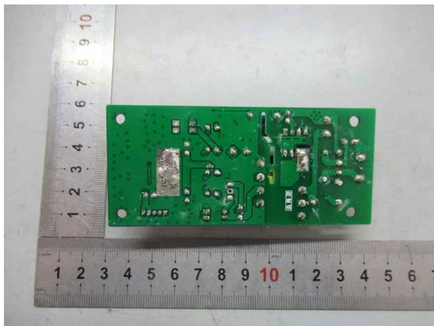
EUT – PCB-1 Bottom View-Main Unit
