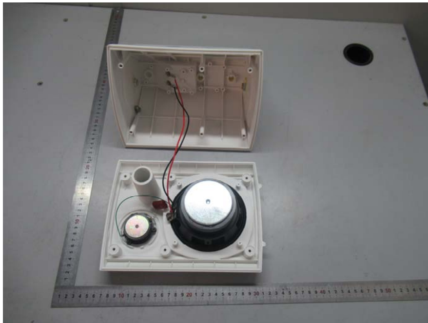
EUT – Cover off View-2- Spraker Unit
