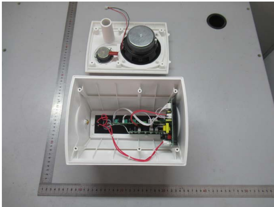
EUT – Cover off View-2-Main Unit
