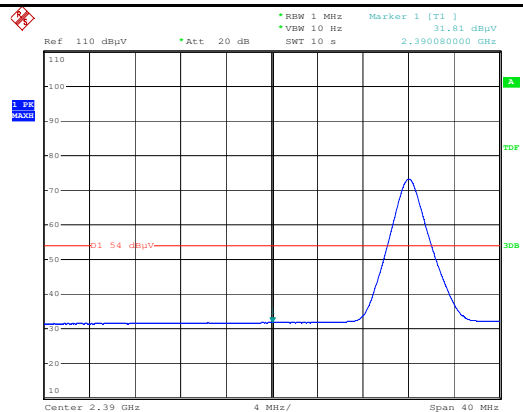
GFSK-Hopping Peak-H
