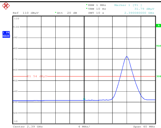
GFSK-Hopping Peak-V
