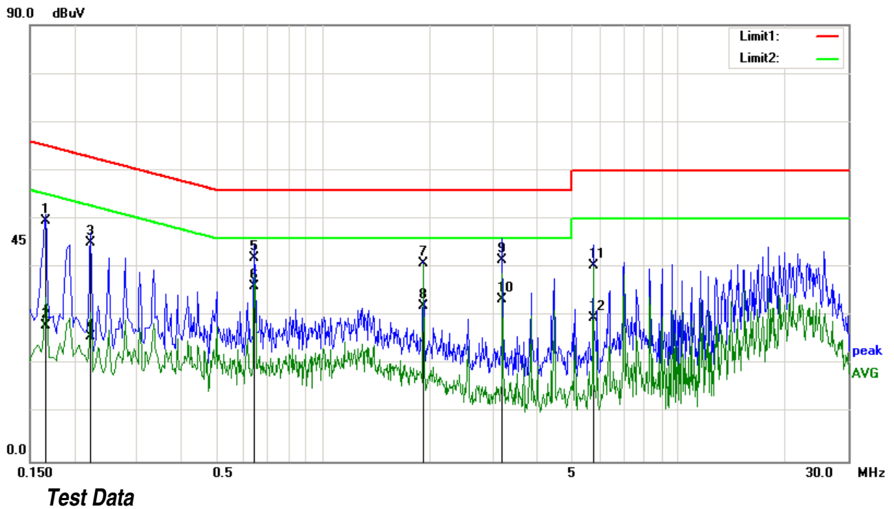
Phase Neutral Plot at AC 240V 50Hz
