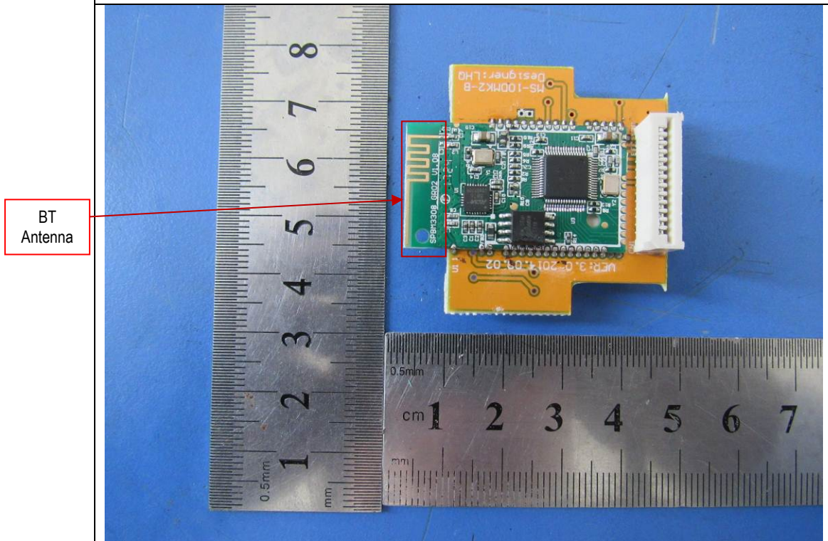
EUT PCB1 – Front View
