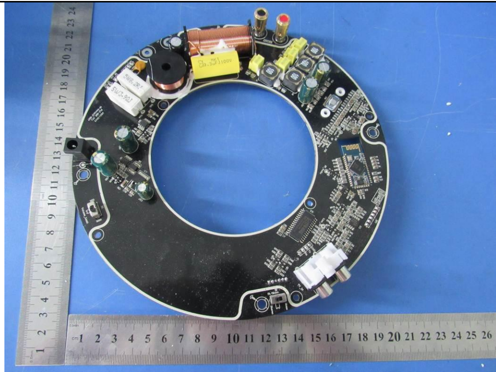
Master Part - PCB Front View
