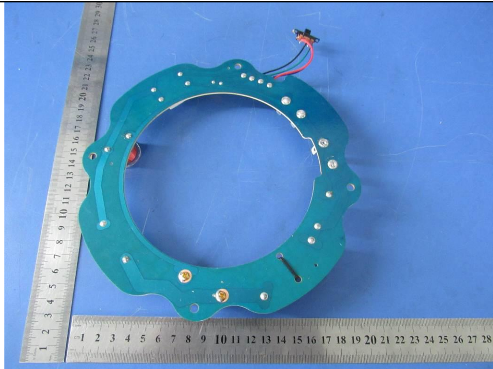
Slave Part - PCB Rear View
