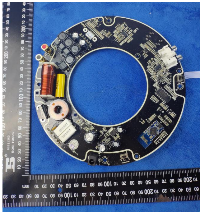
Mainboard-Front View
