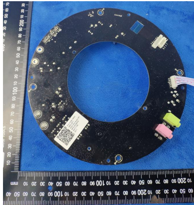
Mainboard-Rear View
