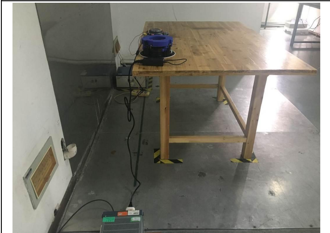
Conducted Emissions Test Setup Side View
