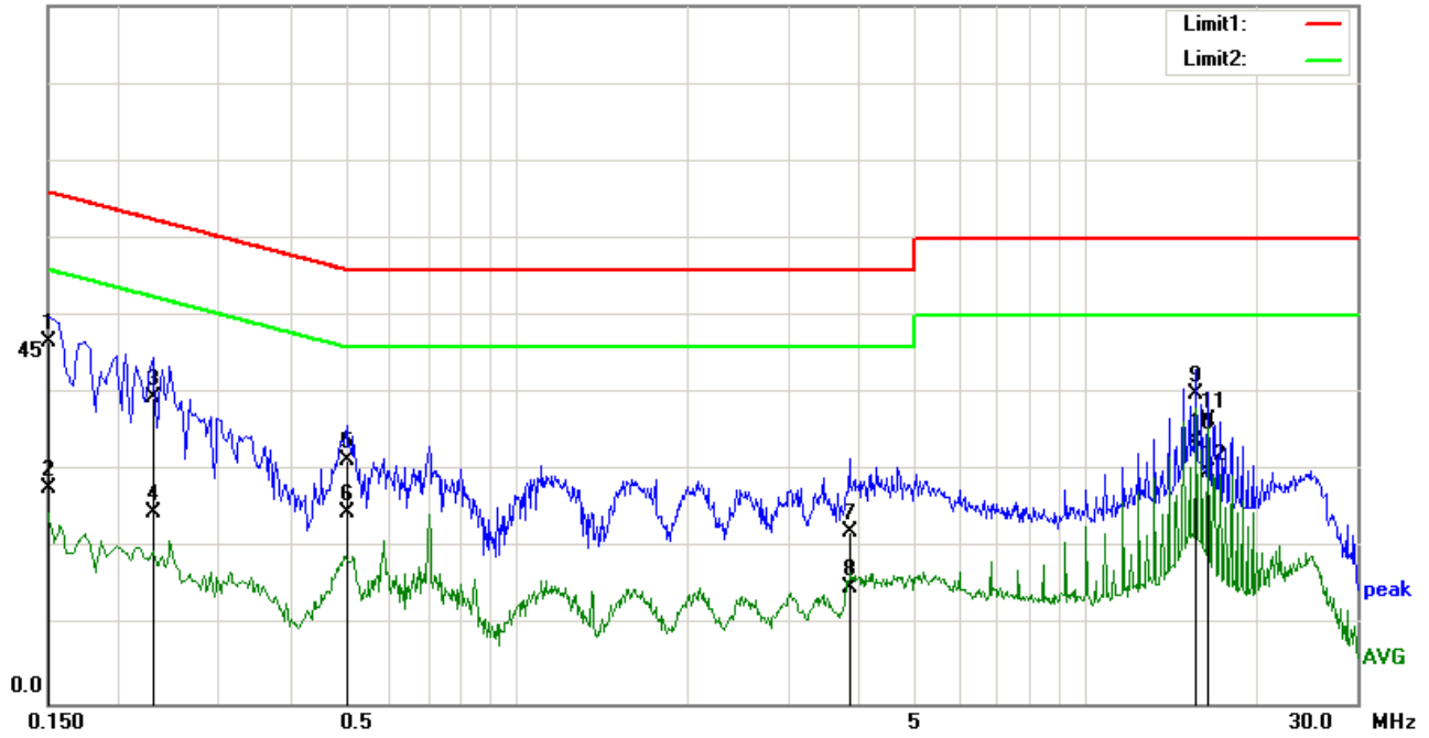
Phase Line Plot at 230Vac, 60Hz
