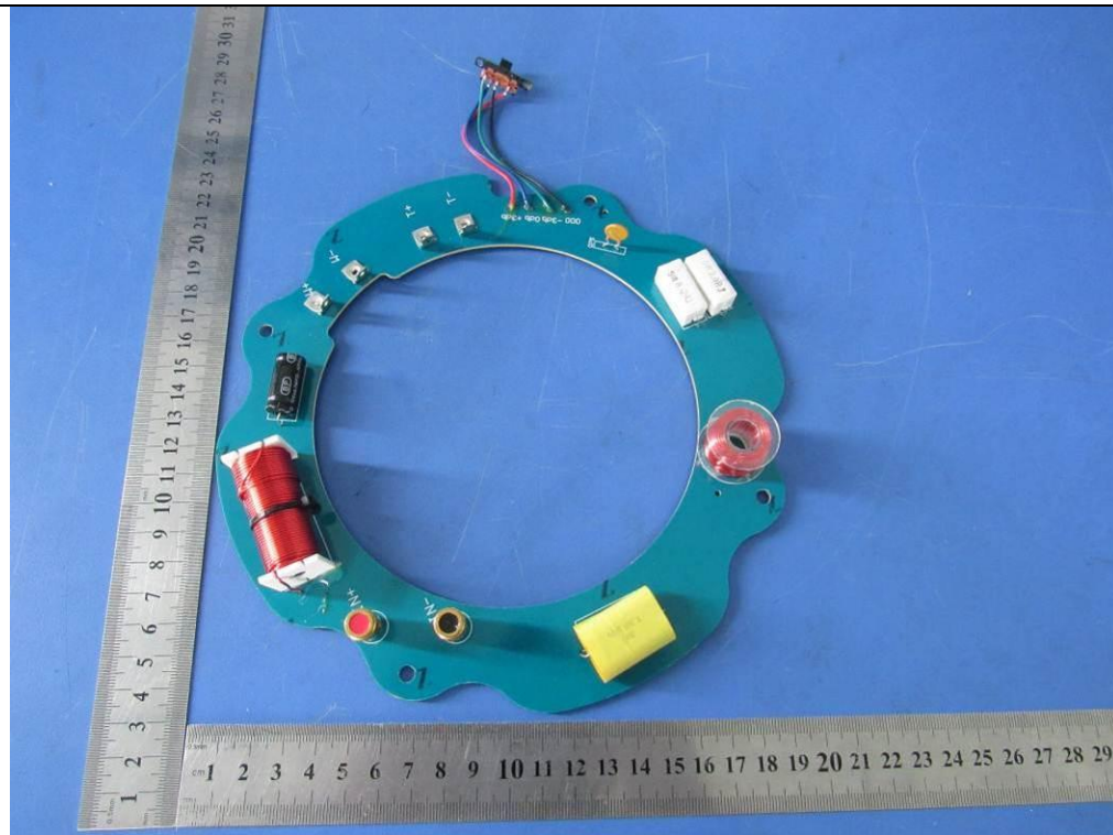
Slave Part - PCB Front View
