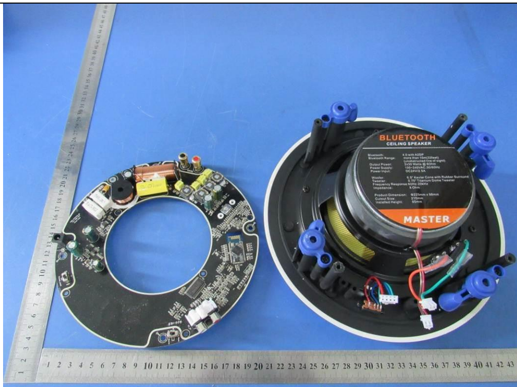
Master Part - Uncover Front View
