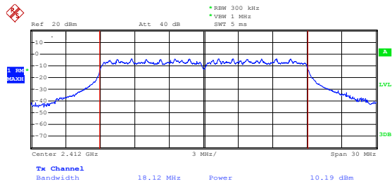
ANT 1(802.11n20)
