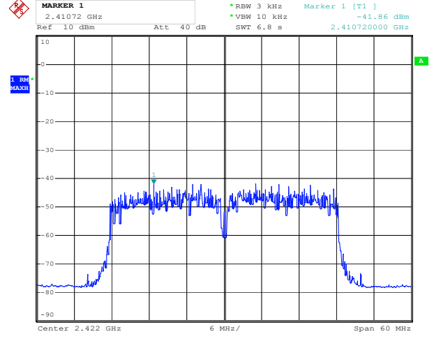
ANT 2(802.11n40)
