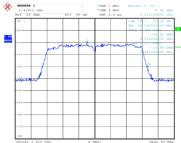
ANT 2(802.11n40)
