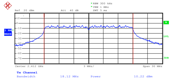
ANT 2(802.11 n20)
