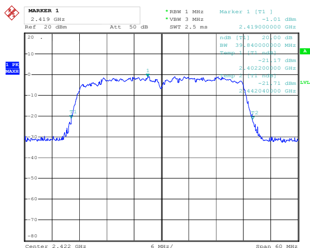
ANT 1(802.11n40)
