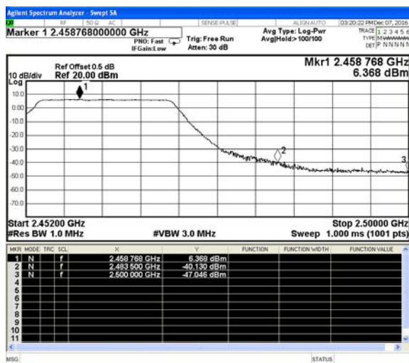
802.11n(HT20)-High channel(Peak)
