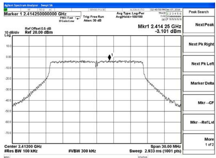
802.11g-Low channel
