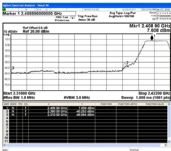
802.11g-Low channel(Peak)
