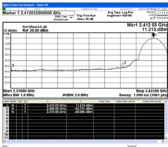
802.11b-Low channel(Peak)
