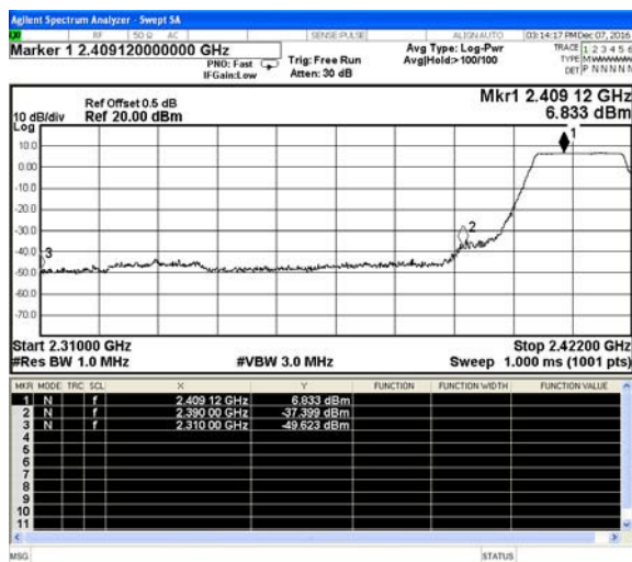
802.11n(HT20)-Low channel(Peak)
