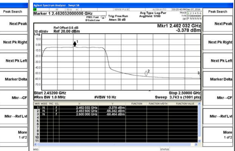
802.11n(HT20)-High channel(Average)
