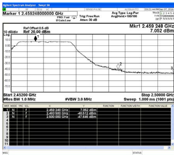
802.11g-High channel(Peak)
