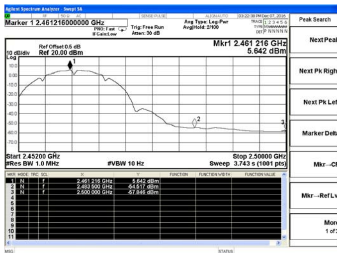
802.11b-High channel(Average)
