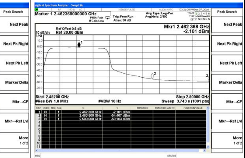
802.11g-High channel(Average)
