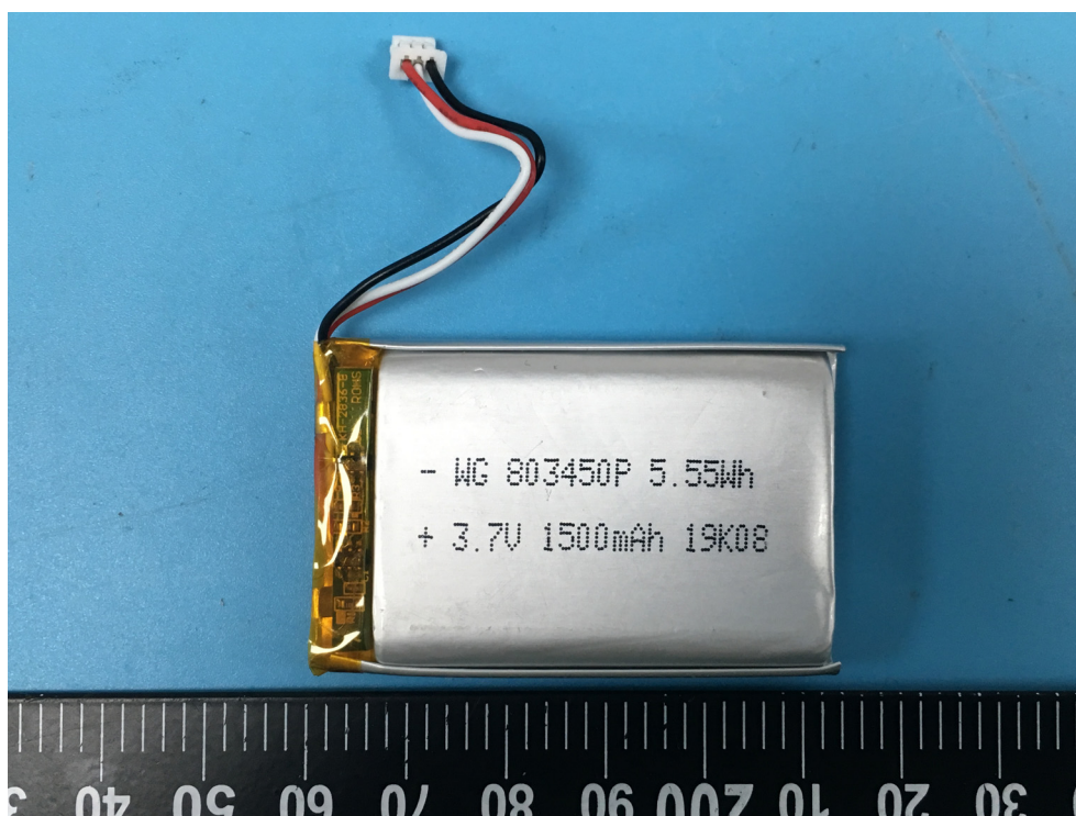
Battery
