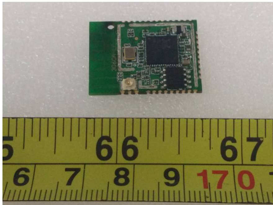
EUT –Cover off Front View 2
