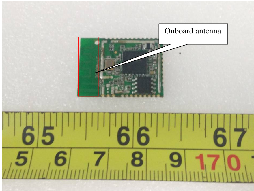
EUT –Cover off Front View 1
