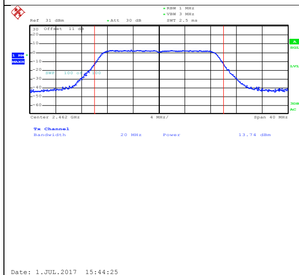
Highest channel
