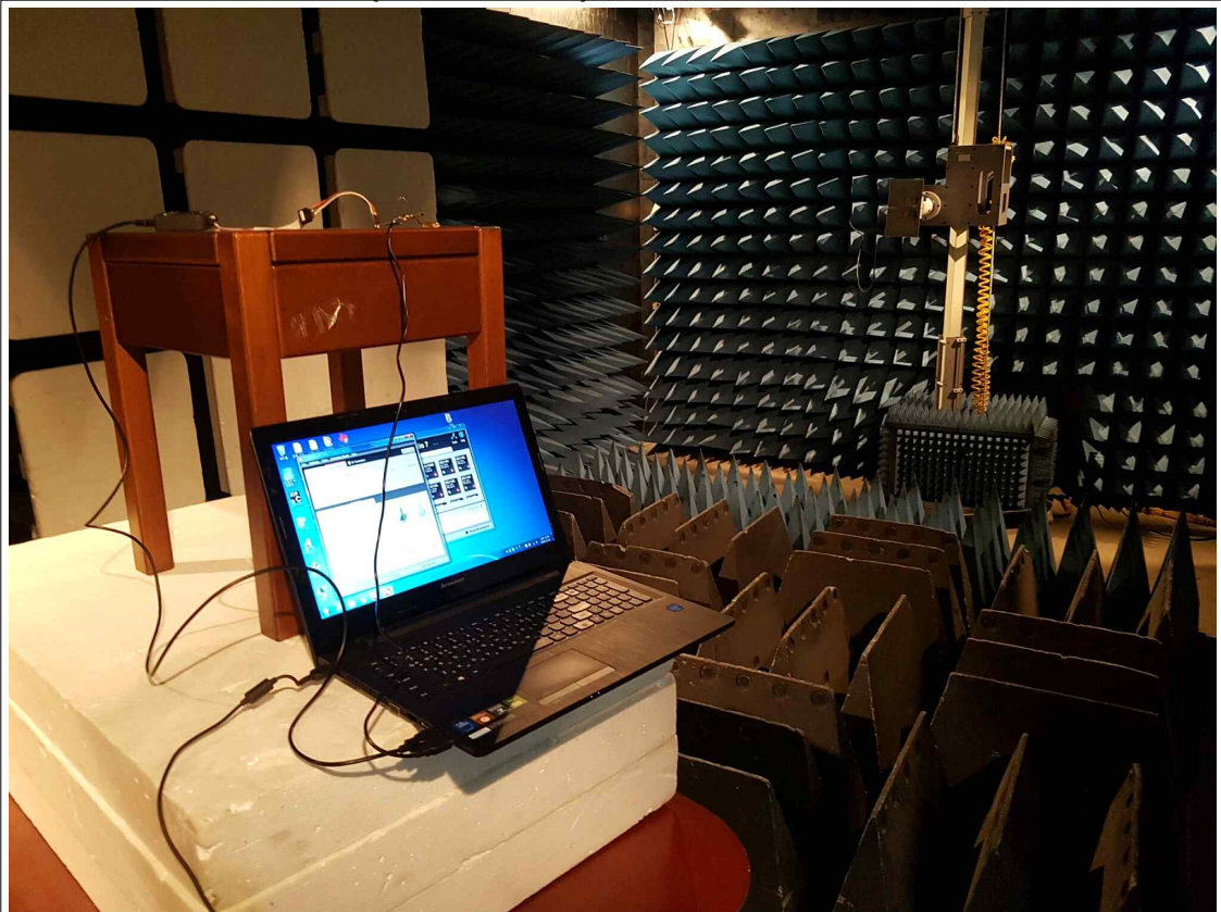
Radiated emission Test (Above 1 GHz)
