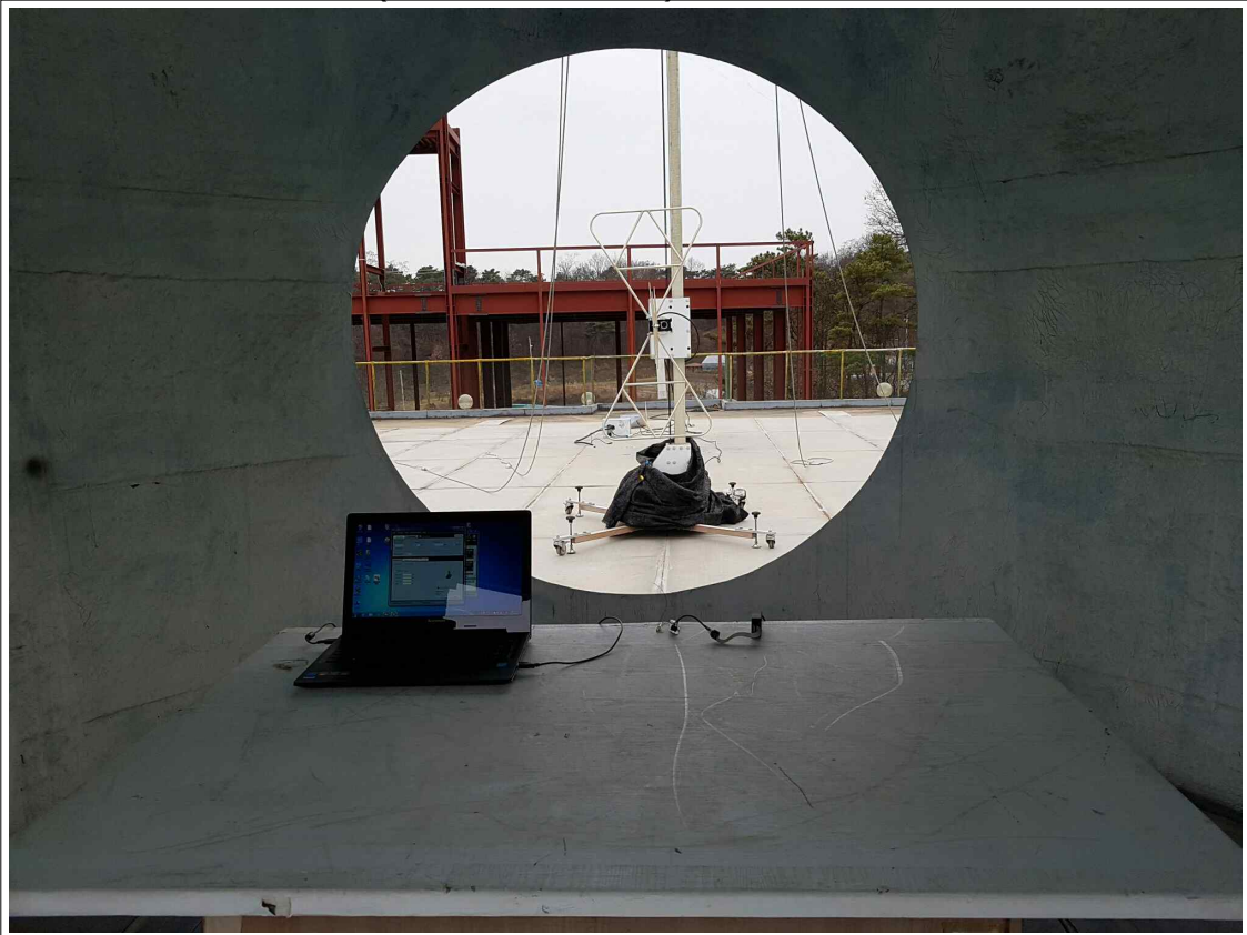
Radiated emission Test (30 MHz to 1 GHz)
