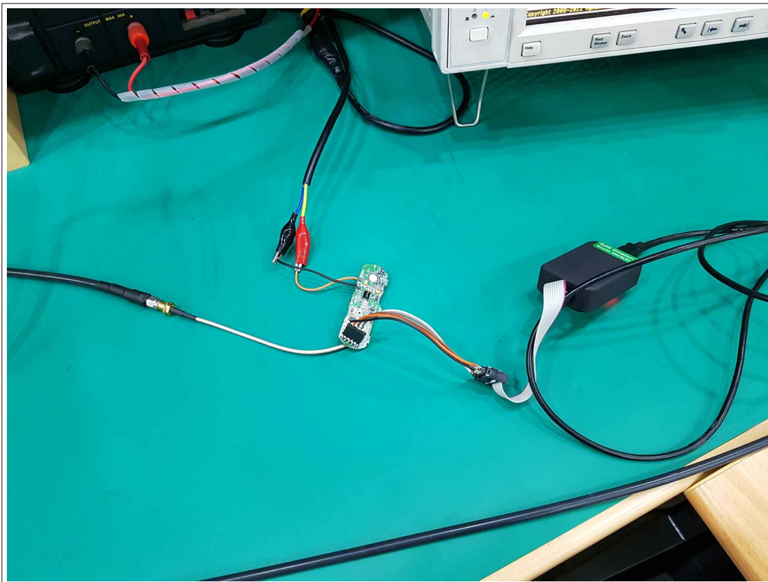
RF conducted emission Test
