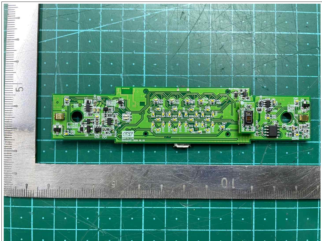
View of PCB (Top)
