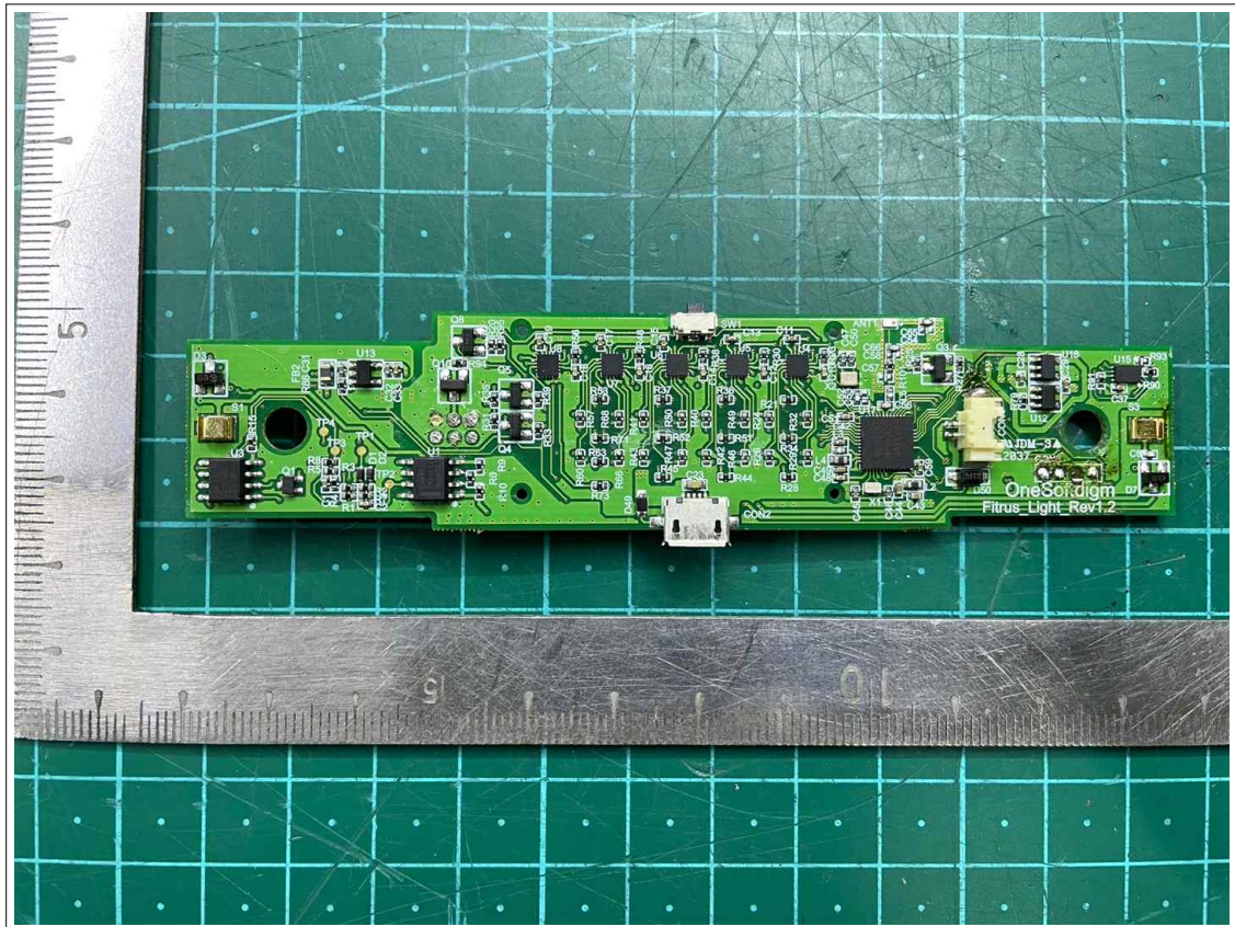
View of PCB (Bottom)
