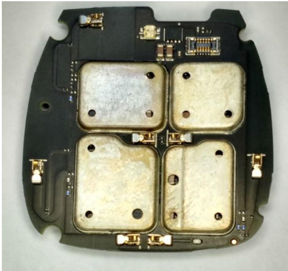
PCB Top Side
