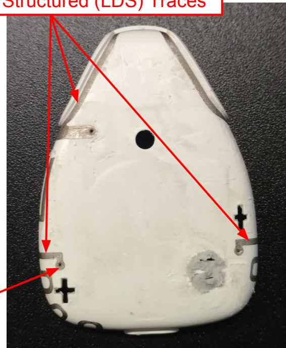
Laser Direct Structured (LDS) Traces
