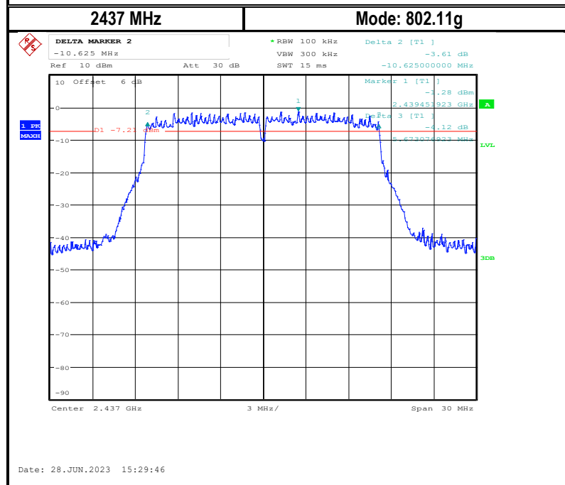
Plot #5
