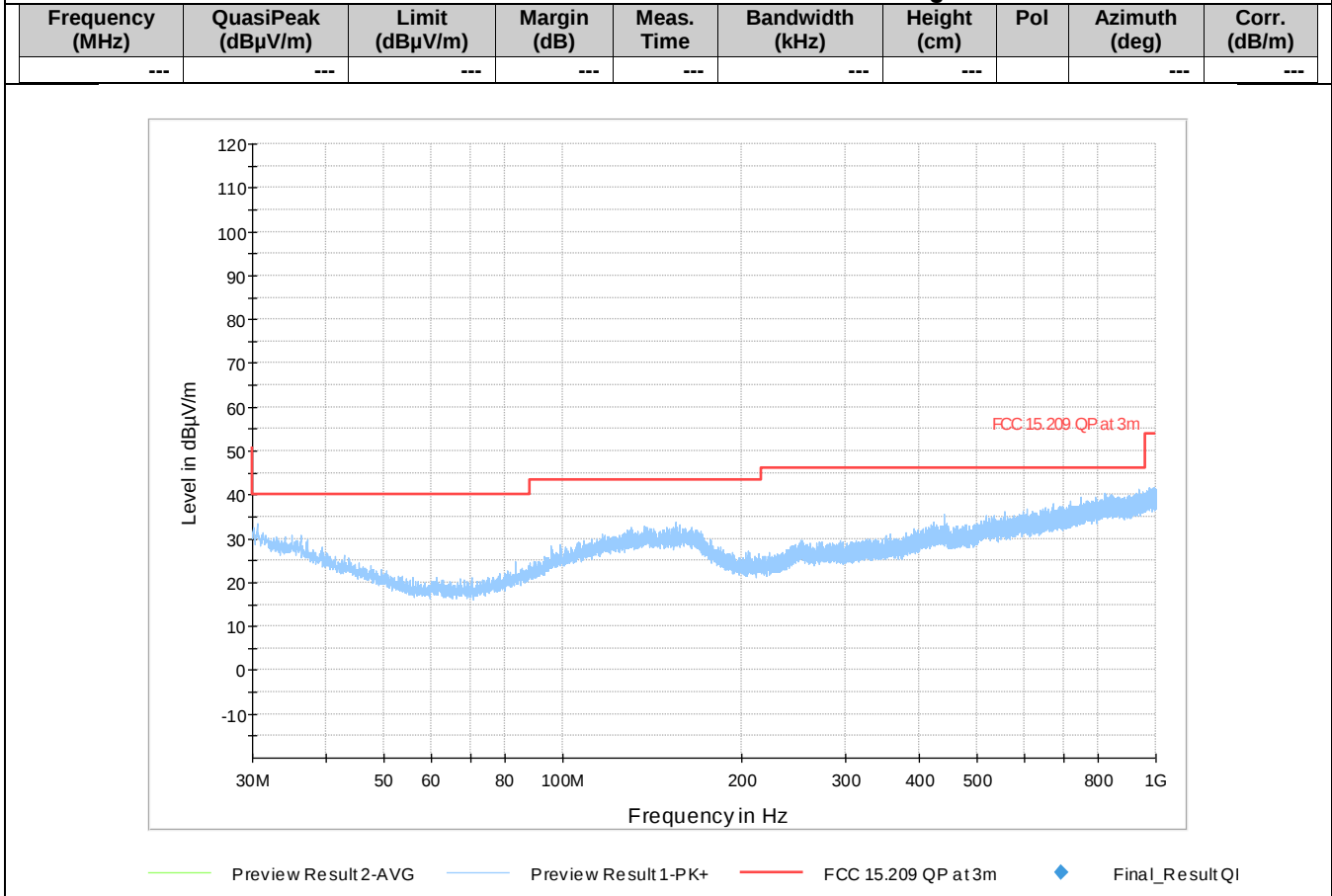
Plot # 9 Radiated Emission 30MHz – 1000MHz High Ch
