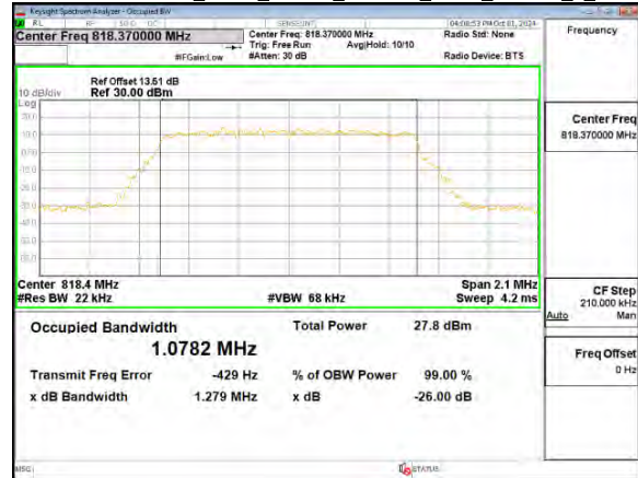
Band26-Part90s_5MHz_Chain0_819MHz_NBI_1_QPSK_6_0
