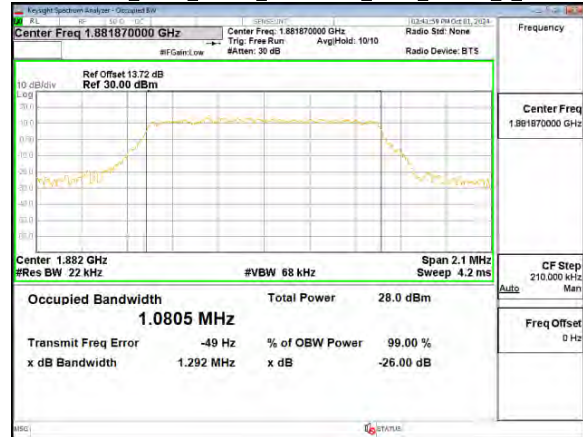
Band25_5MHz_Chain0_1882.5MHz_NBI_1_QPSK_6_0
