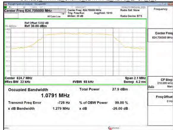
Band26_1.4MHz_Chain0_824.7MHz_NBI 0_QPSK_6_0
