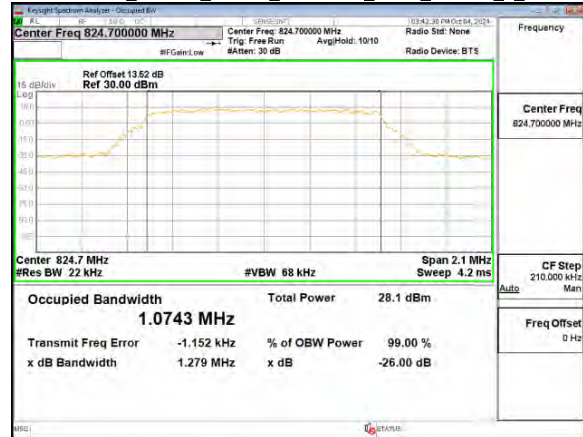
Band26_1.4MHz_Chain0_824.7MHz_NBI 0_QPSK_6_0
