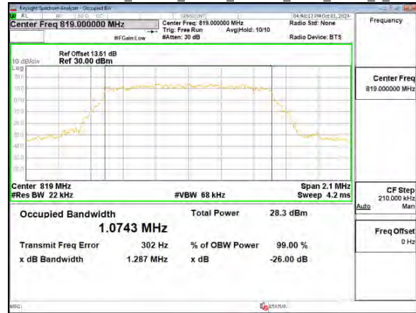
Band26-Part90s_1.4MHz_Chain0_819MHz_NBI 0_QPSK_6_0
