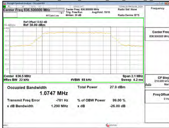
Band26_1.4MHz_Chain0_836.5MHz_NBI 0_QPSK_6_0
