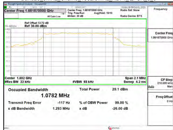
Band25_5MHz_Chain0_1882.5MHz_NBI_1_QPSK_6_0
