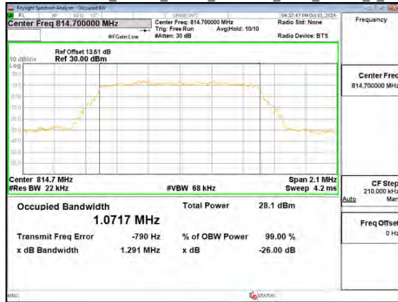
Band26-Part90s_1.4MHz_Chain0_814.7MHz_NBI 0_16QAM_6_0
