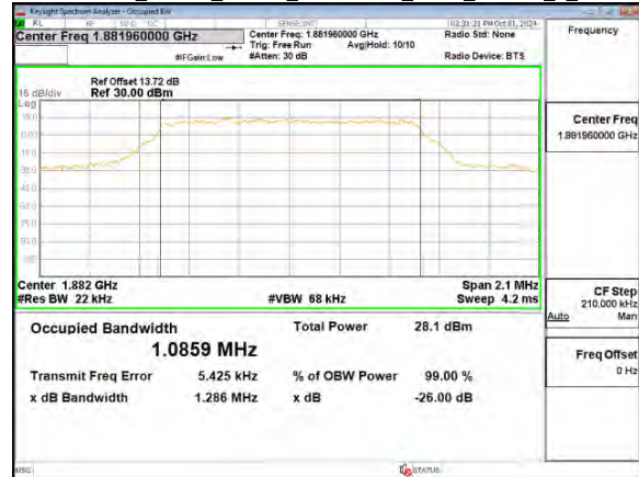
Band25_10MHz_Chain0_1882.5MHz_NBI 3_QPSK_6_0
