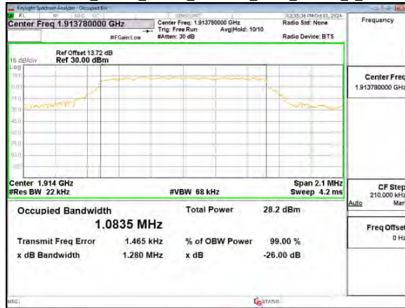
Band25_10MHz_Chain0_1910MHz_NBI 7_QPSK_6_0
