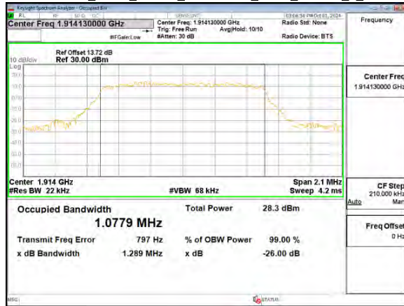
Band25_3MHz_Chain0_1913.5MHz_NBI_1_QPSK_6_0
