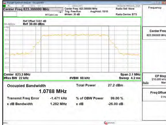
Band26-Part90s_1.4MHz_Chain0_823.3MHz_NBI 0_QPSK_6_0
