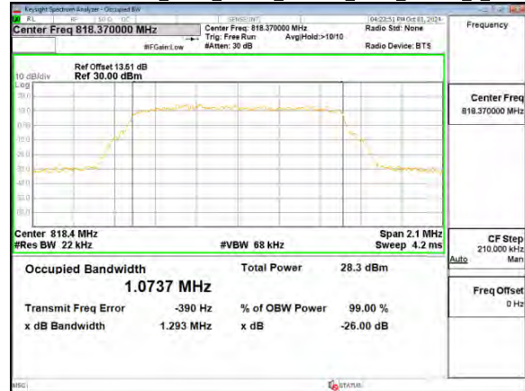
Band26-Part90s_3MHz_Chain0_819MHz_NBI 0_QPSK_6_0
