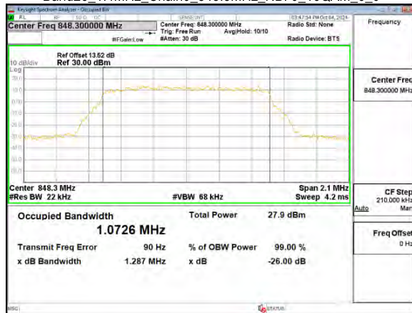
Band26_1.4MHz_Chain0_848.3MHz_NBI 0_16QAM_6_0
