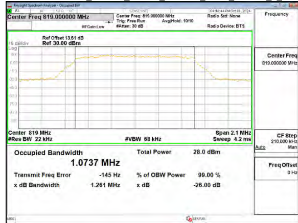
Band26-Part90s_1.4MHz_Chain0_819MHz_NBI 0_QPSK_6_0
