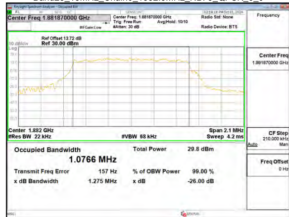
Band25_15MHz_Chain0_1882.5MHz_NBI 5_QPSK_6_0
