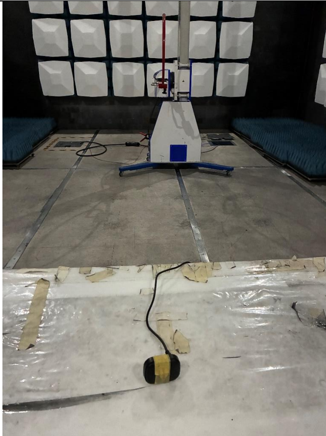
9kHz – 30MHz Rear View
