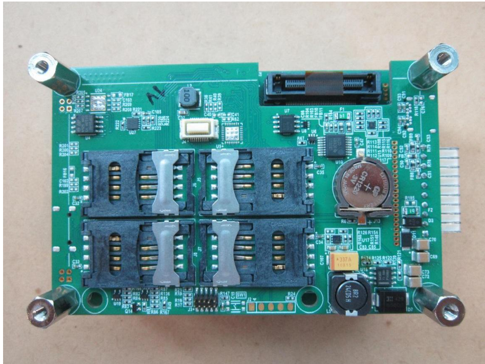
Sub-Board - Front View
