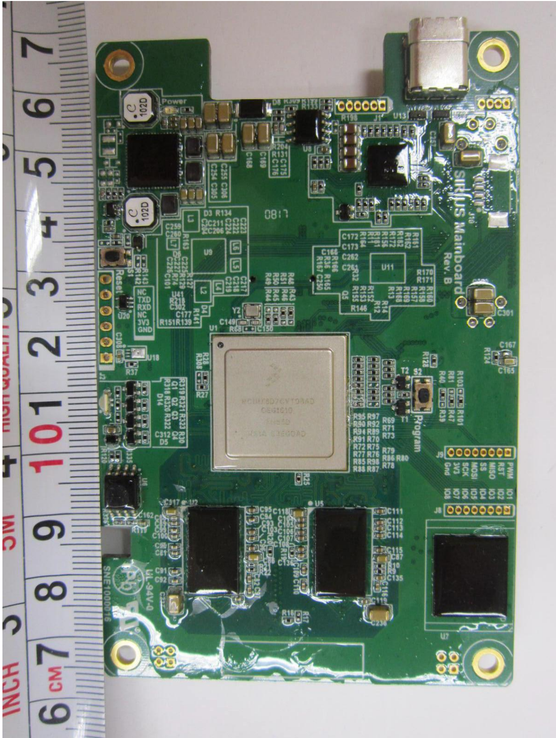
Module Board PCB Trace View
