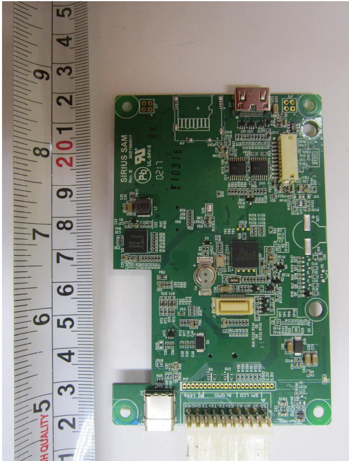
Main-Board PCB Trace View
