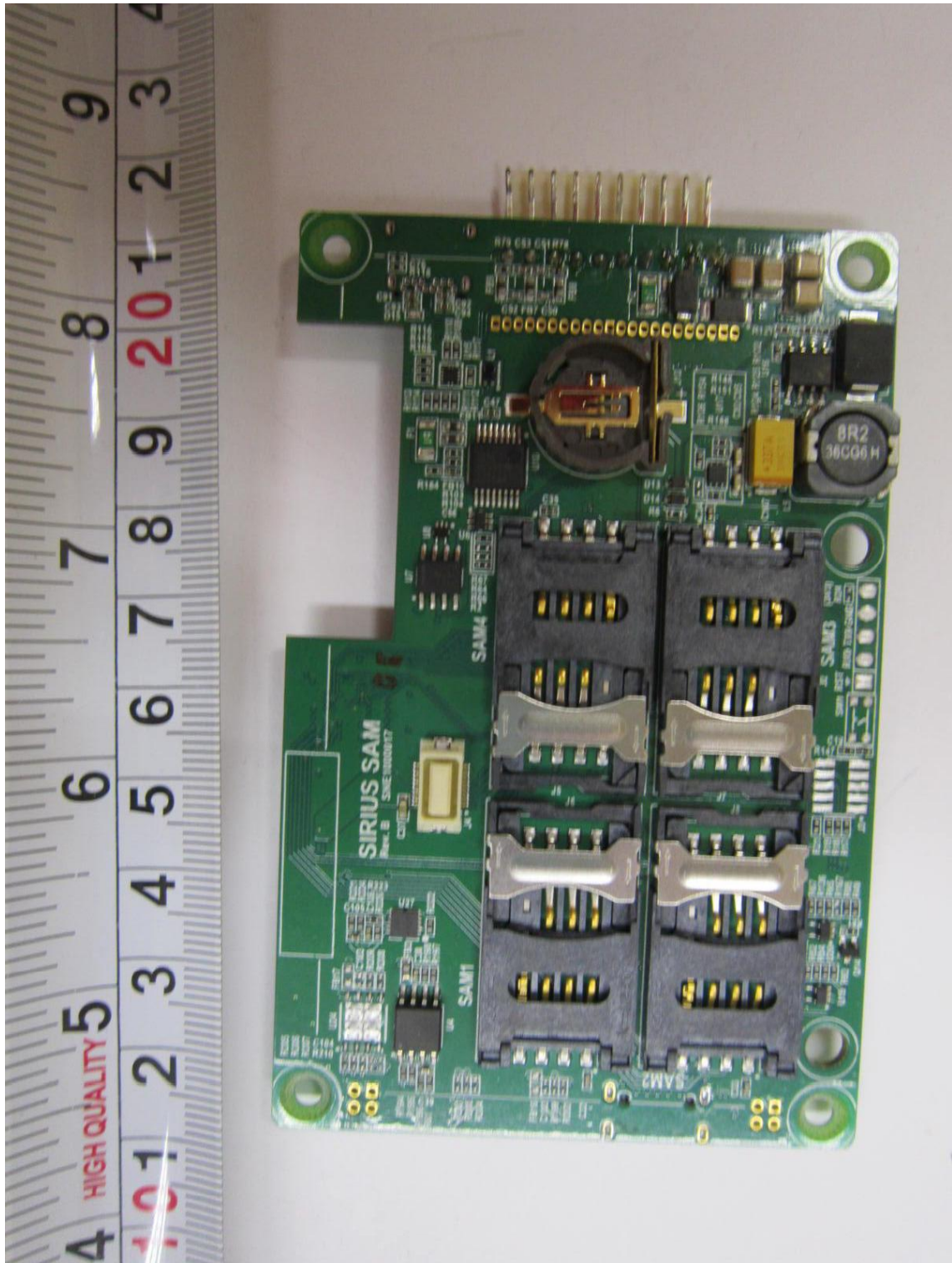
Main-Board PCB Component View
