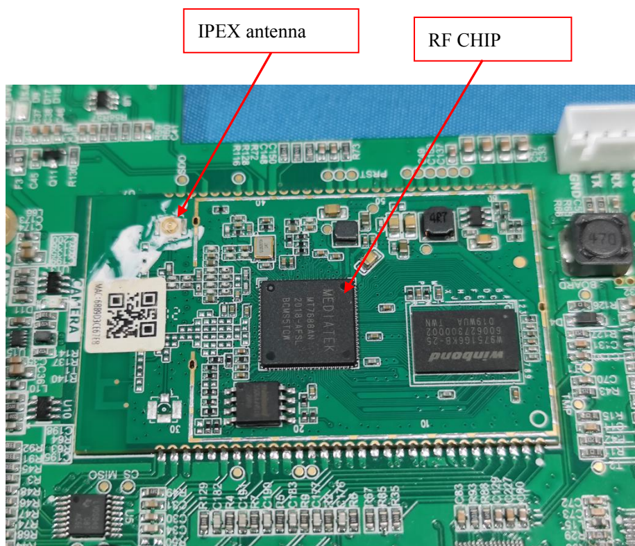
RF CHIP: Model : MT7688AN Manufacturer:MEDIATEK
