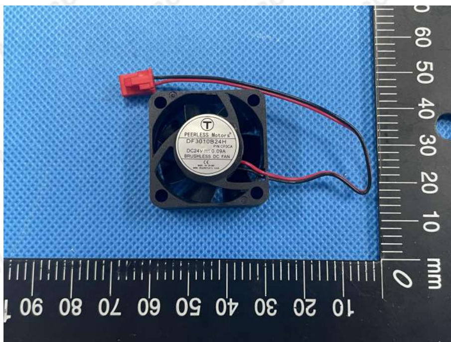
DF3010B24H-CF0CA
