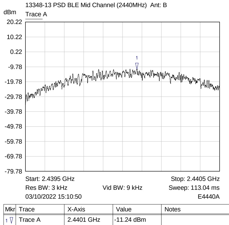
Plot for AVGPSD-1 Result
