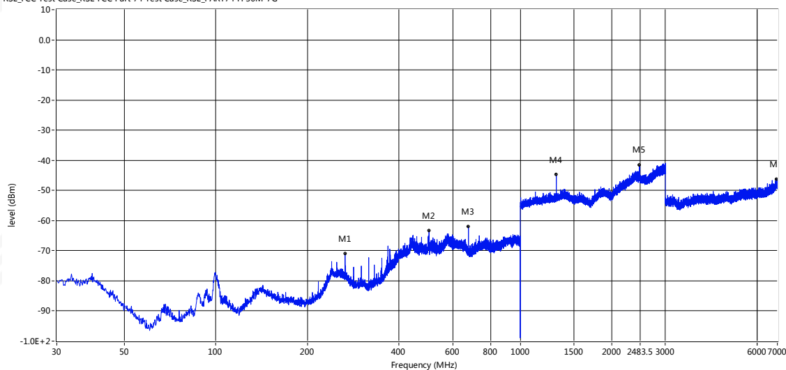
RSE_FCC Test Case_RSE FCC Part 74 Test Case_RSE_PART74 H 30M-7G
