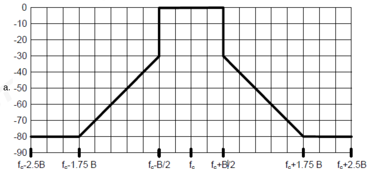
Figure 2: Transmit spectral power mask for equipment employing digital modulation, except WMA5, RBW = 1 kHz
