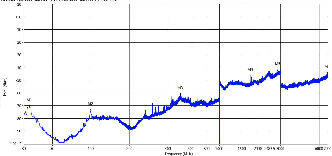
RSE_FCC Test Case_RSE FCC Part 74 Test Case_RSE_PART74 V 30M-7G
