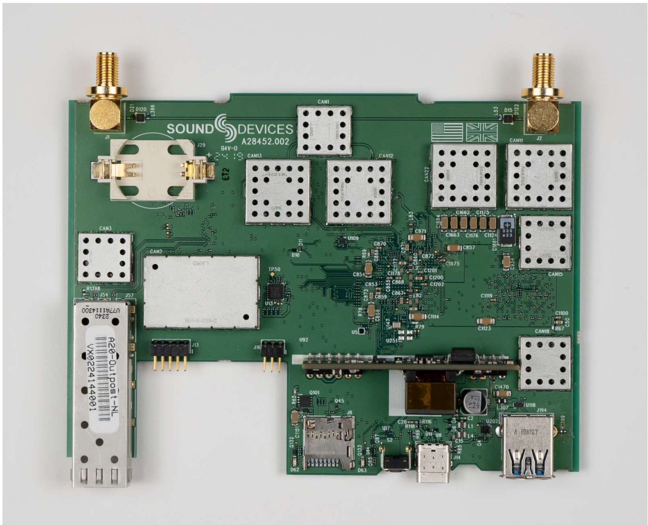
MAIN PCB(TOP)
