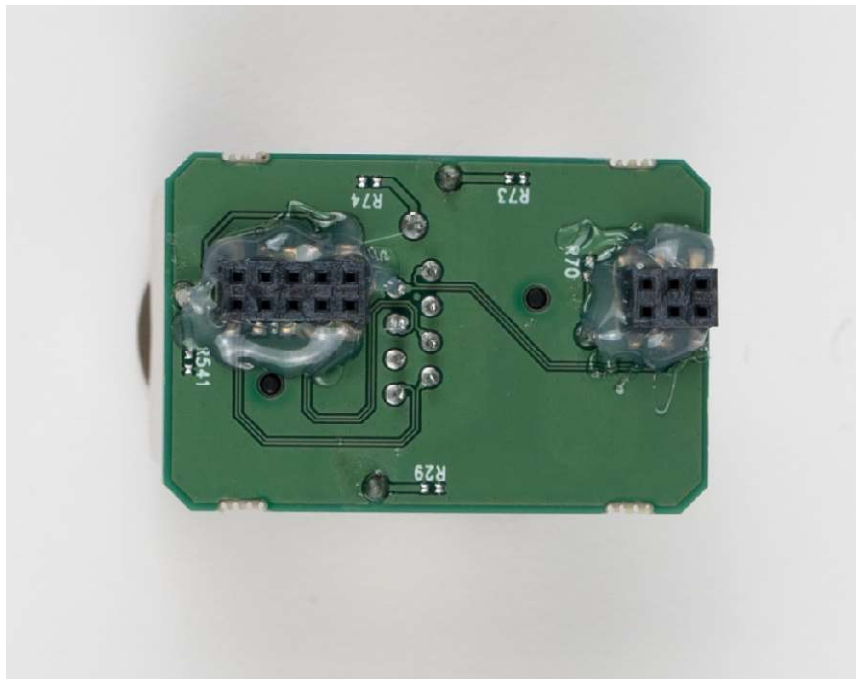
ETHERNET-1 PCB(BOTTOM)
