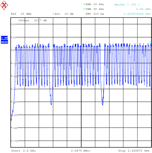
2400 MHz – 2420.875 MHz 49 Channels
