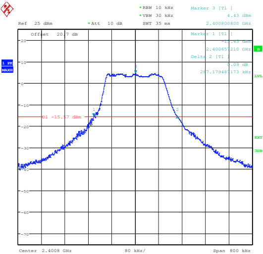
2400.8 MHz
