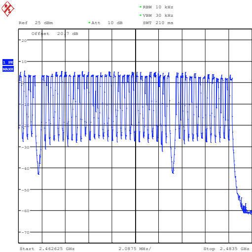
2462.625 MHz-2483.5 MHz 46 Channels
