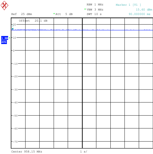
958.15 MHz
