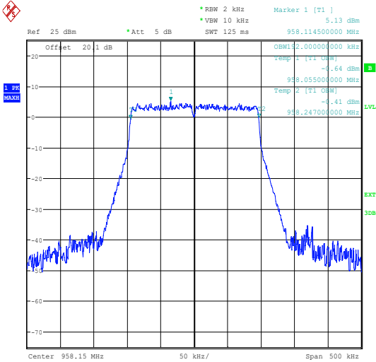
958.15 MHz
