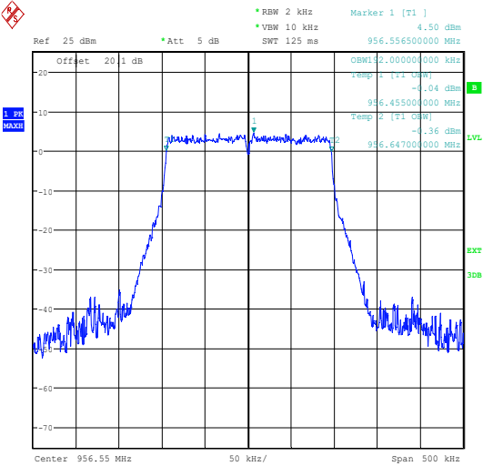
956.55 MHz
