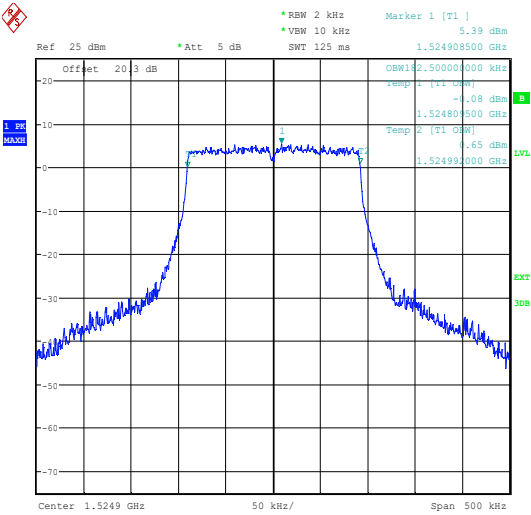
1524.9 MHz
