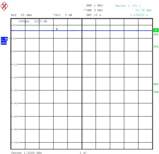
1524.90 MHz
