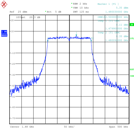
1480.0 MHz
