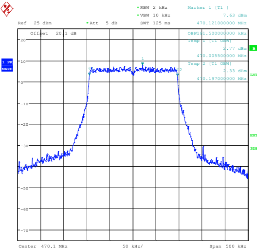
470.1 MHz
