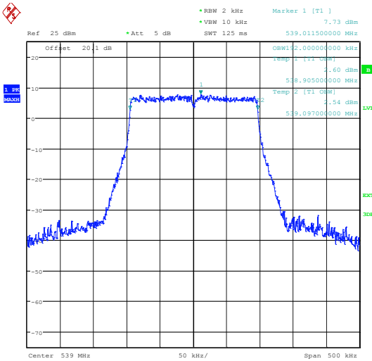
539.0 MHz
