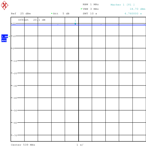
539.00 MHz
