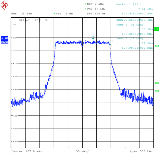
607.9 MHz
