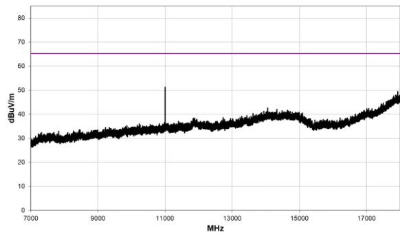
171.875 MHz 7 GHz - 18 GHz
