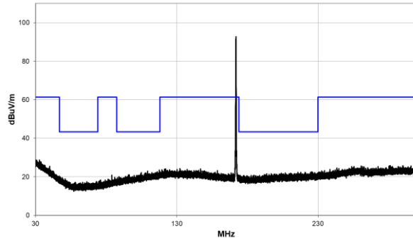
171.875 MHz 30 MHz -300 MHz
