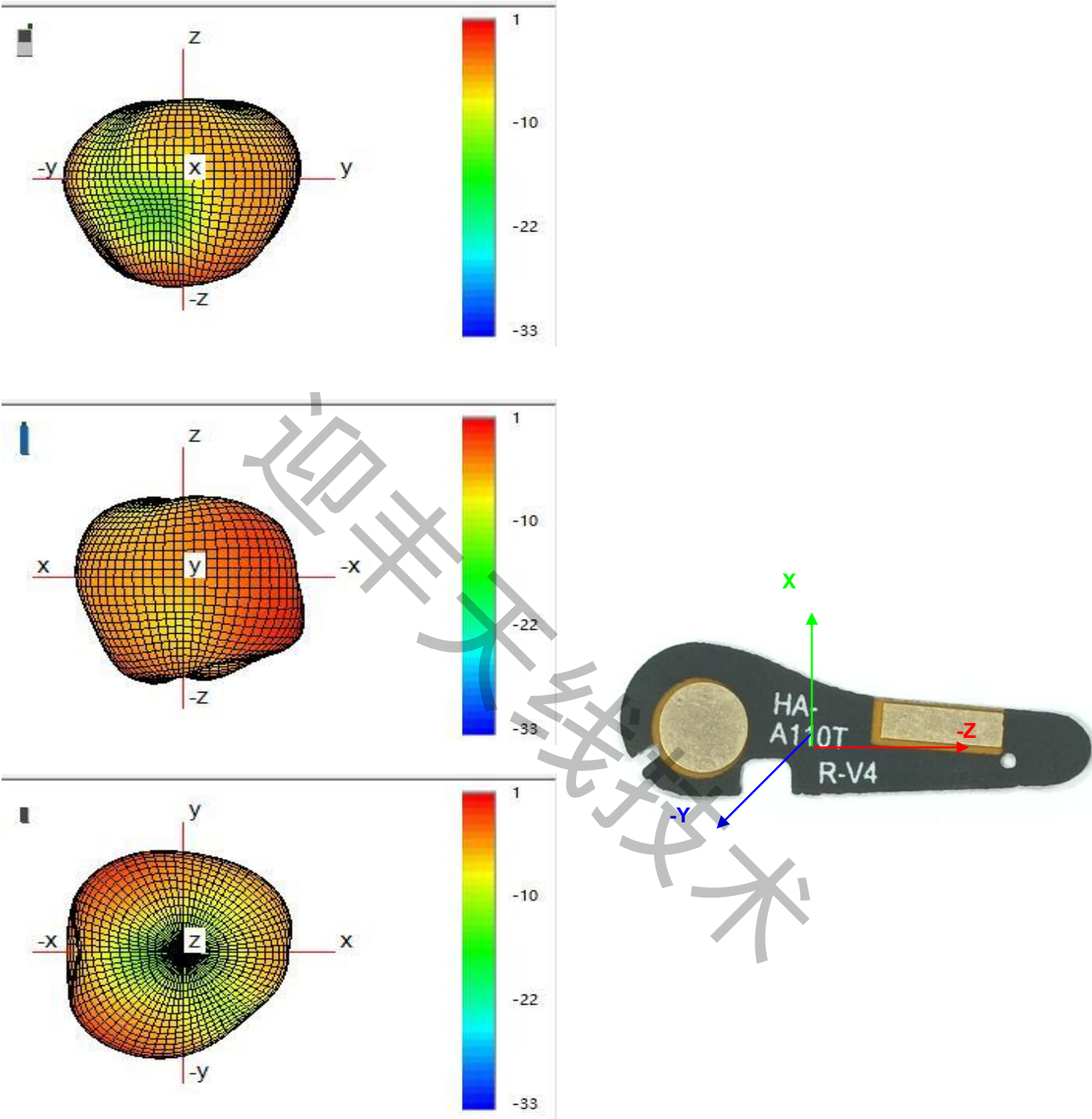
9-1.3D Gain Pattern (Radiation Pattern at 2450 MHz)
